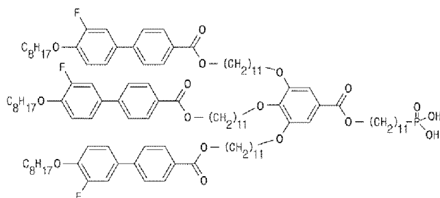
[Structural formula 3]
