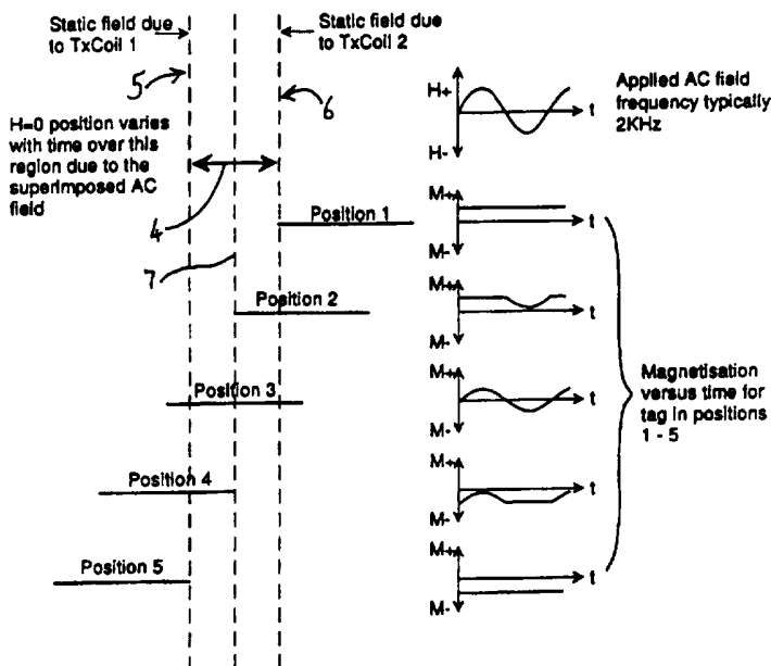
Signals from tag at different positions with respect to null plane
