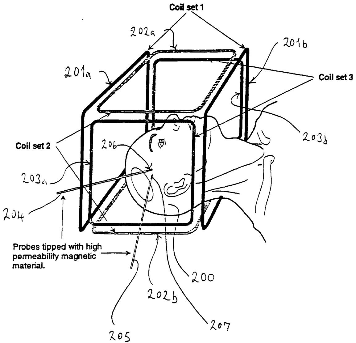
Fig 10: 3-D location system for surgical applications
