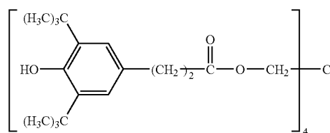
Compound (III-1):
