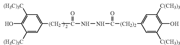
Compound (III-1):
