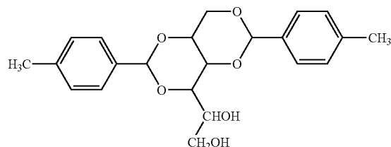
Compound (II-1):
