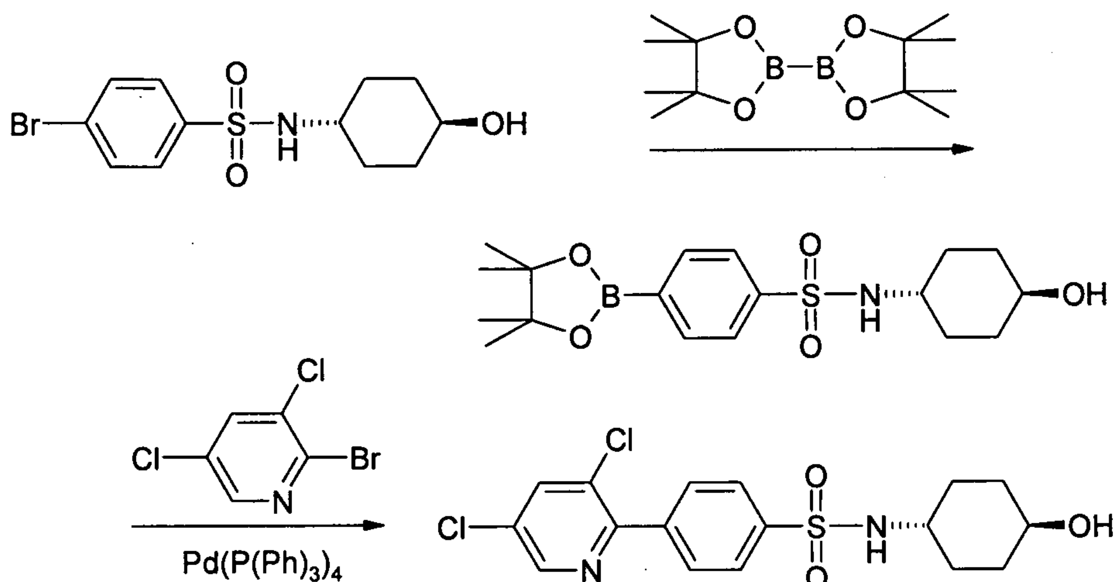
Scheme 18
