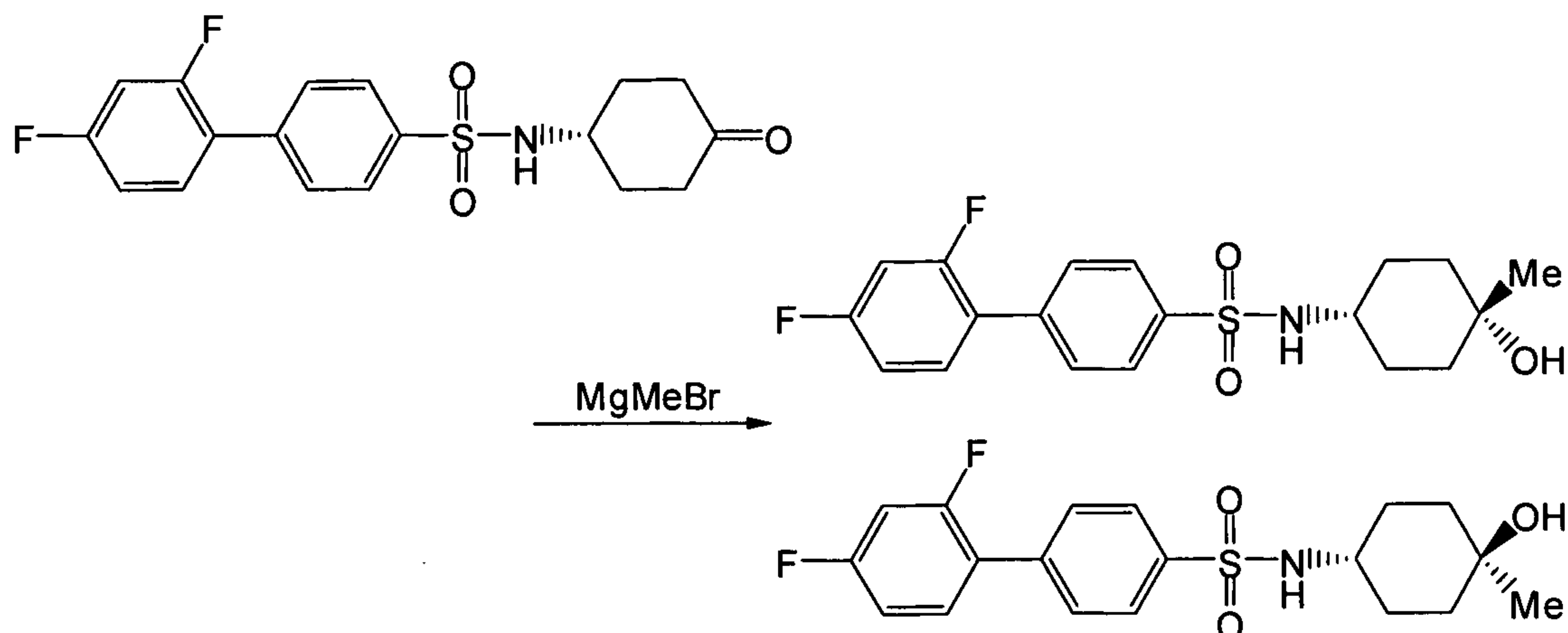
Scheme 15
