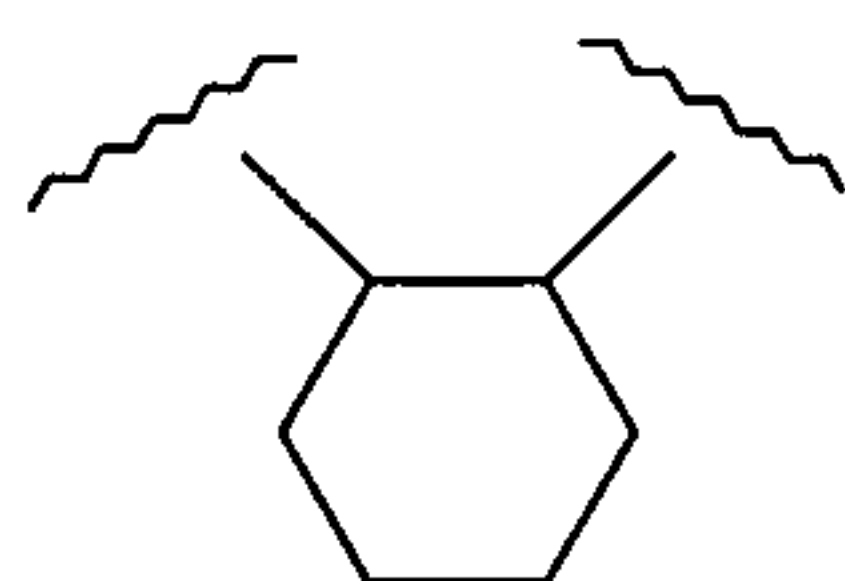
cyclohexane-1,2-di-yl
