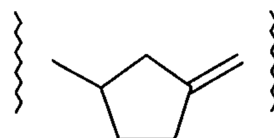
cyclopentane-1-yl-3-ylidene
