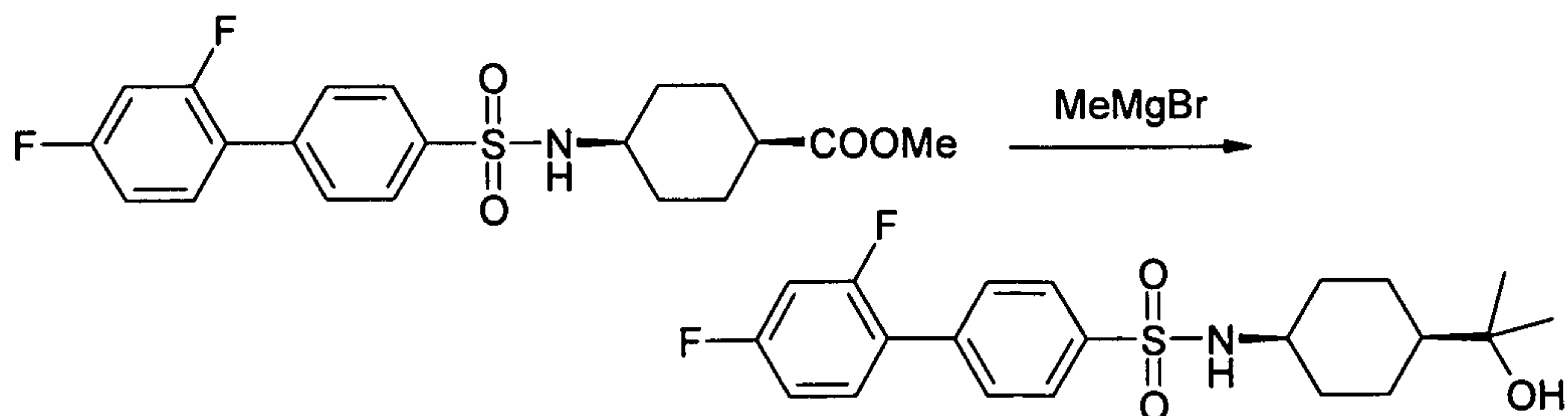
Scheme 17
