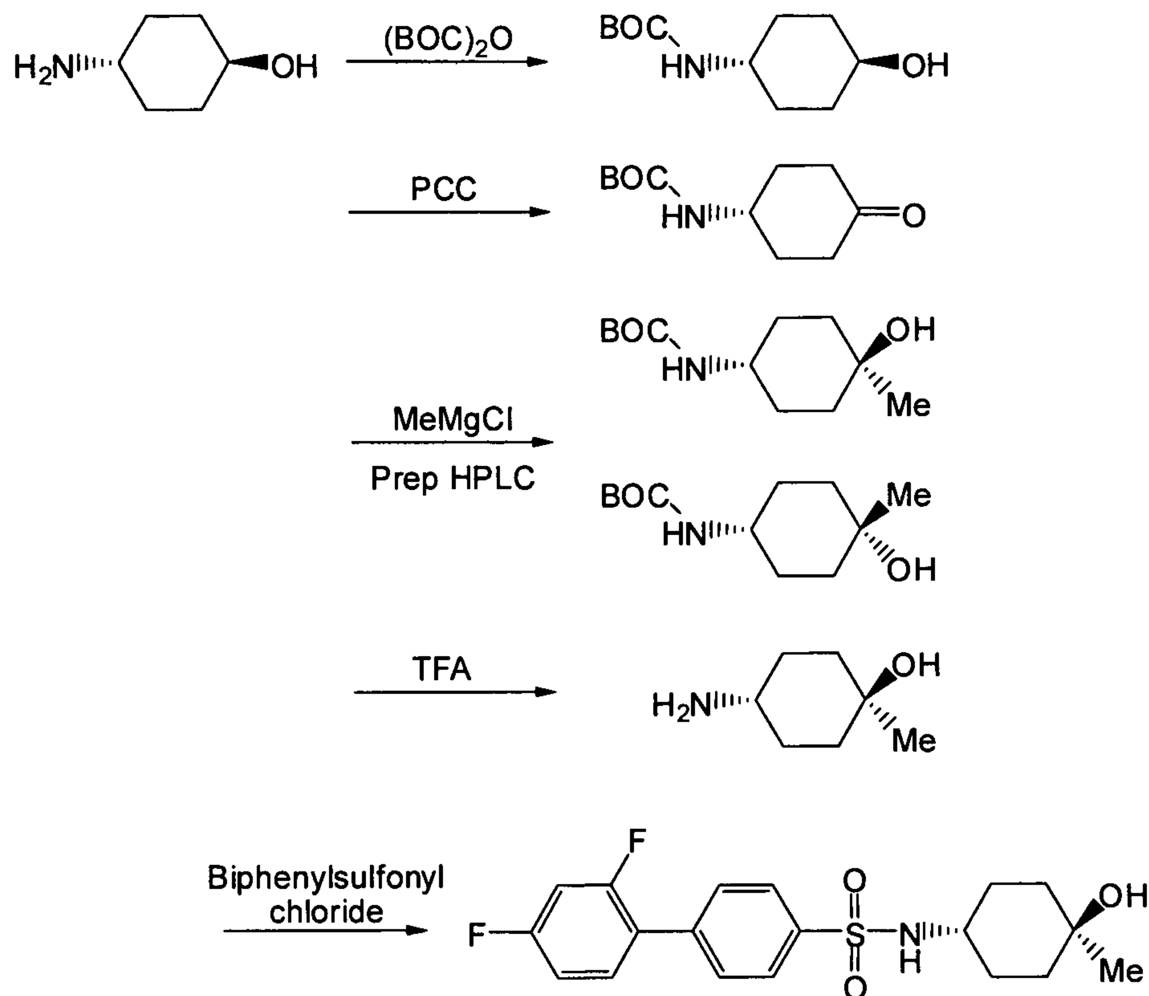
Scheme 16
