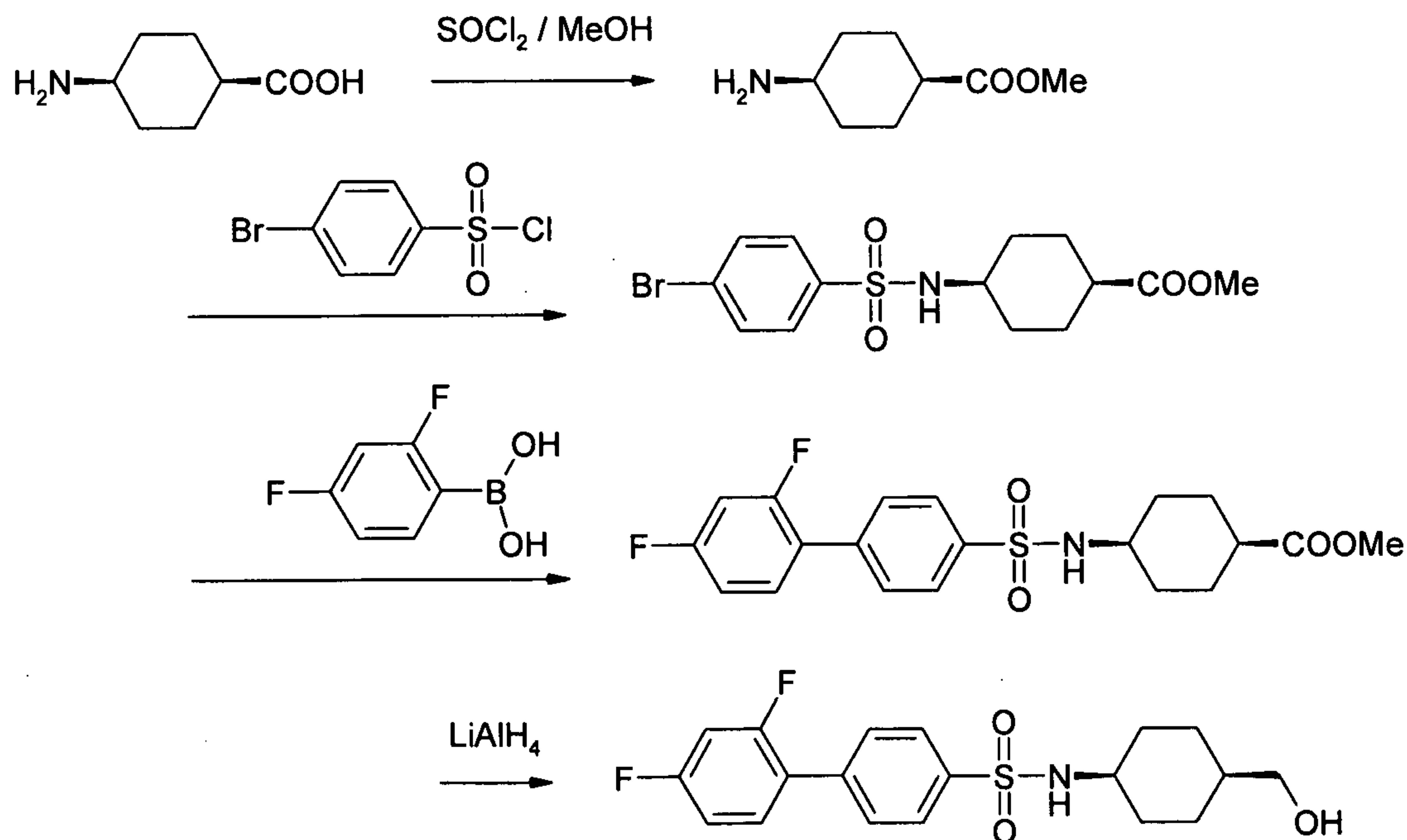
Scheme 3
