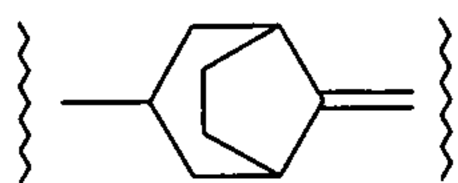
bicyclo[3.2.1]octane-3-yl-8-ylidene
