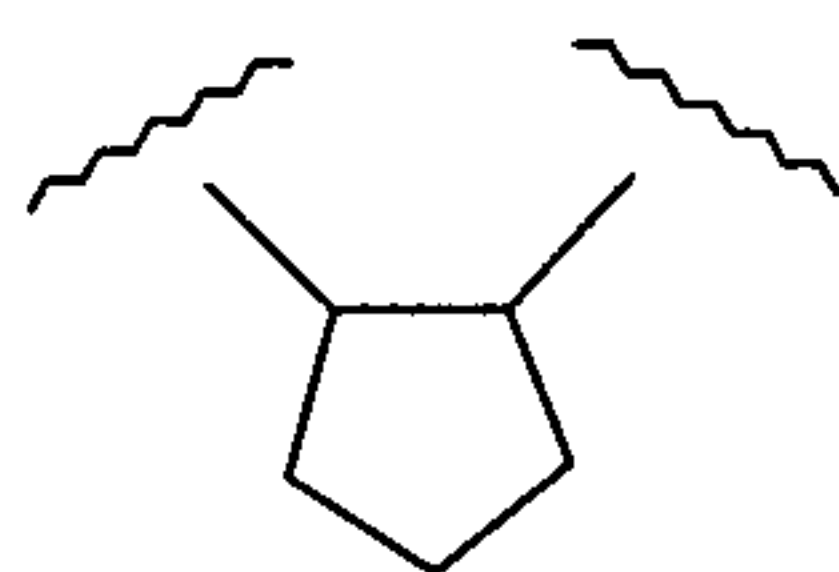
cyclopentane-1,2-di-yl
