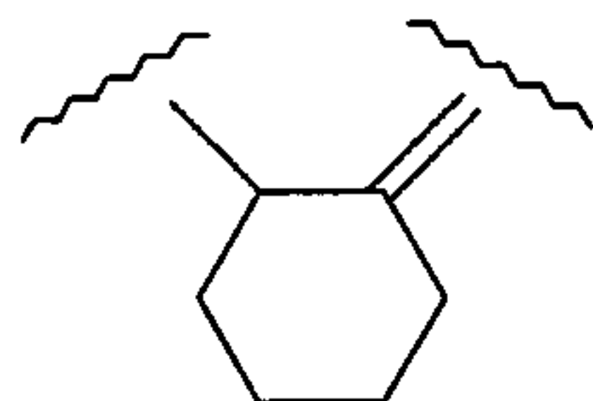
cyclohexane-1-yl-2-ylidene
