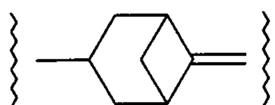
bicyclo[3.1.1]heptane-3-yl-6-ylidene
