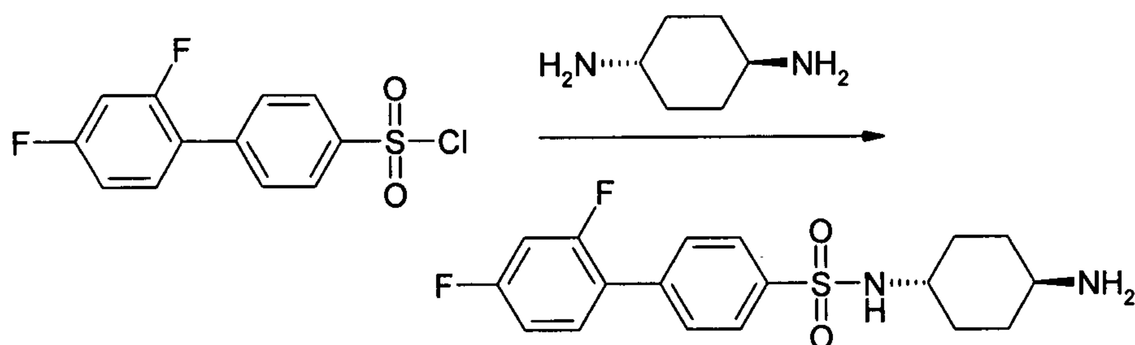
Scheme 10
