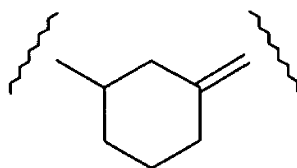
cyclohexane-1-yl-3-ylidene
