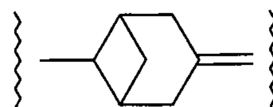
bicyclo[3.1.1]heptane-6-yl-3-ylidene
