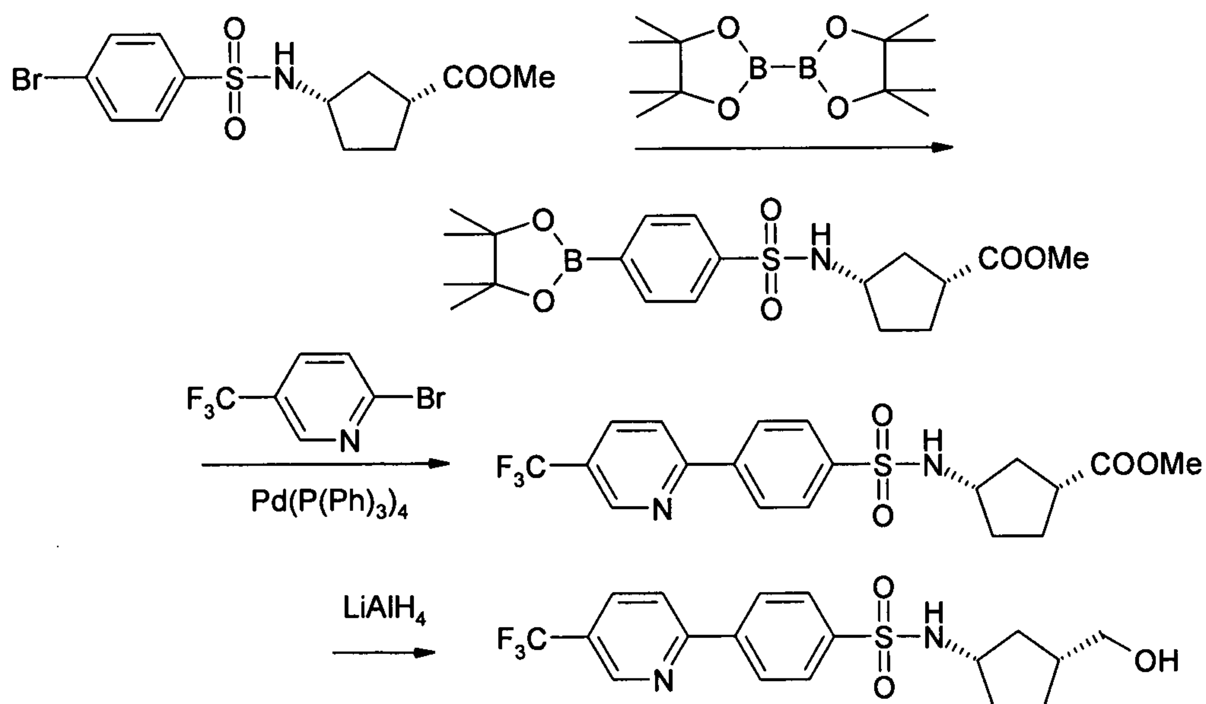
Scheme 19
