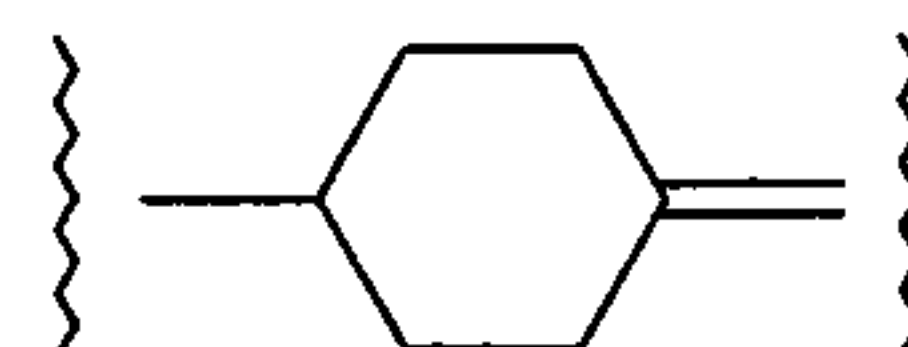
cyclohexane-1-yl-4-ylidene
