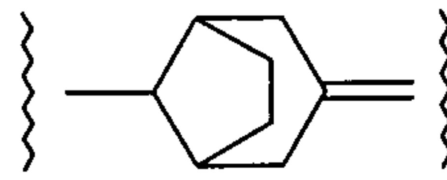
bicyclo[3.2.1]octane-8-yl-3-ylidene
