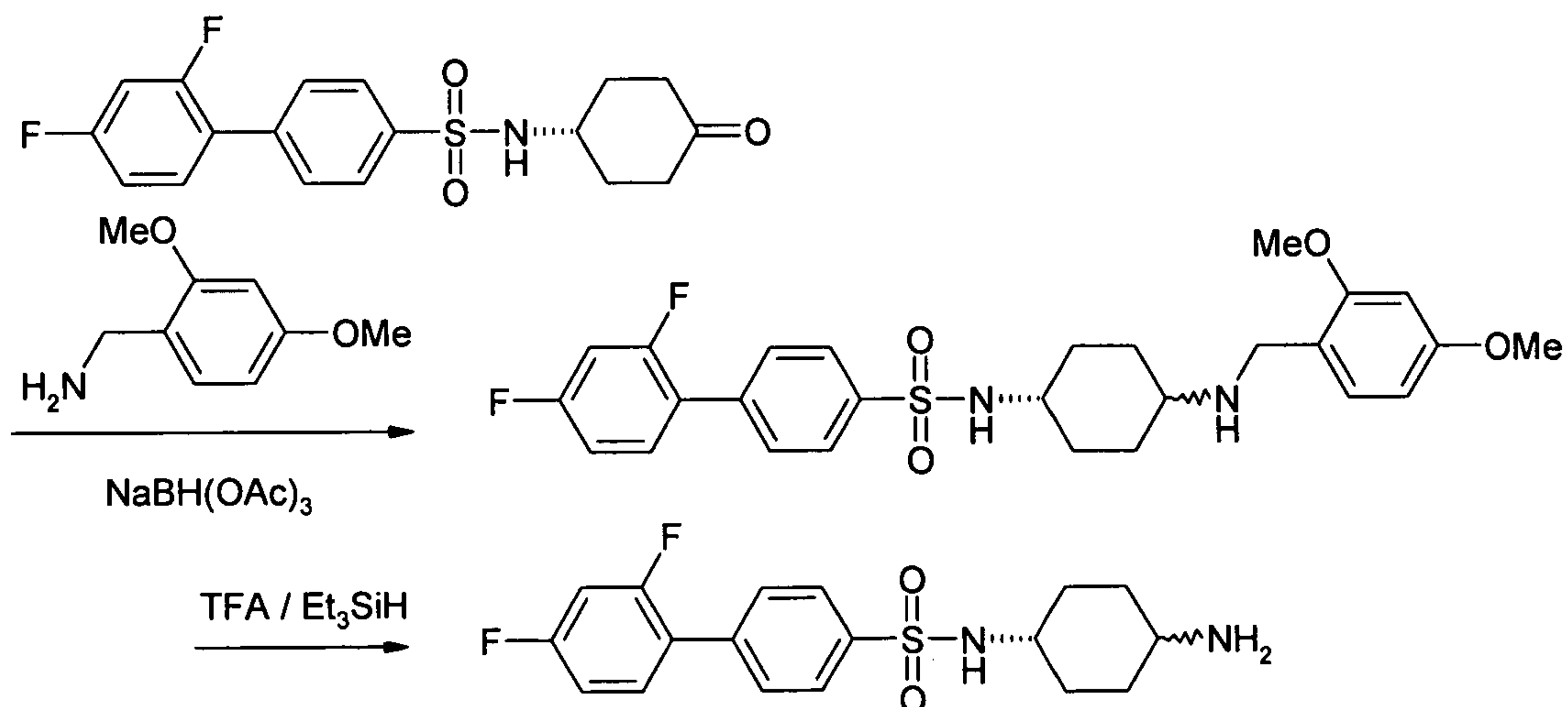
Scheme 12
