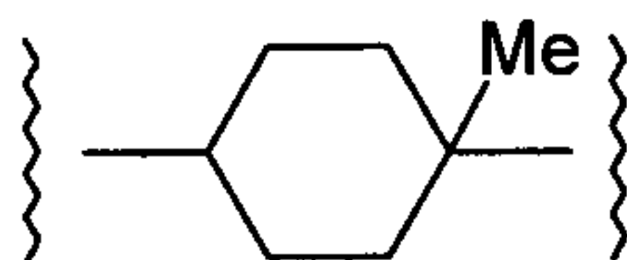
4-methyl-cyclohexane-1,4-di-yl
