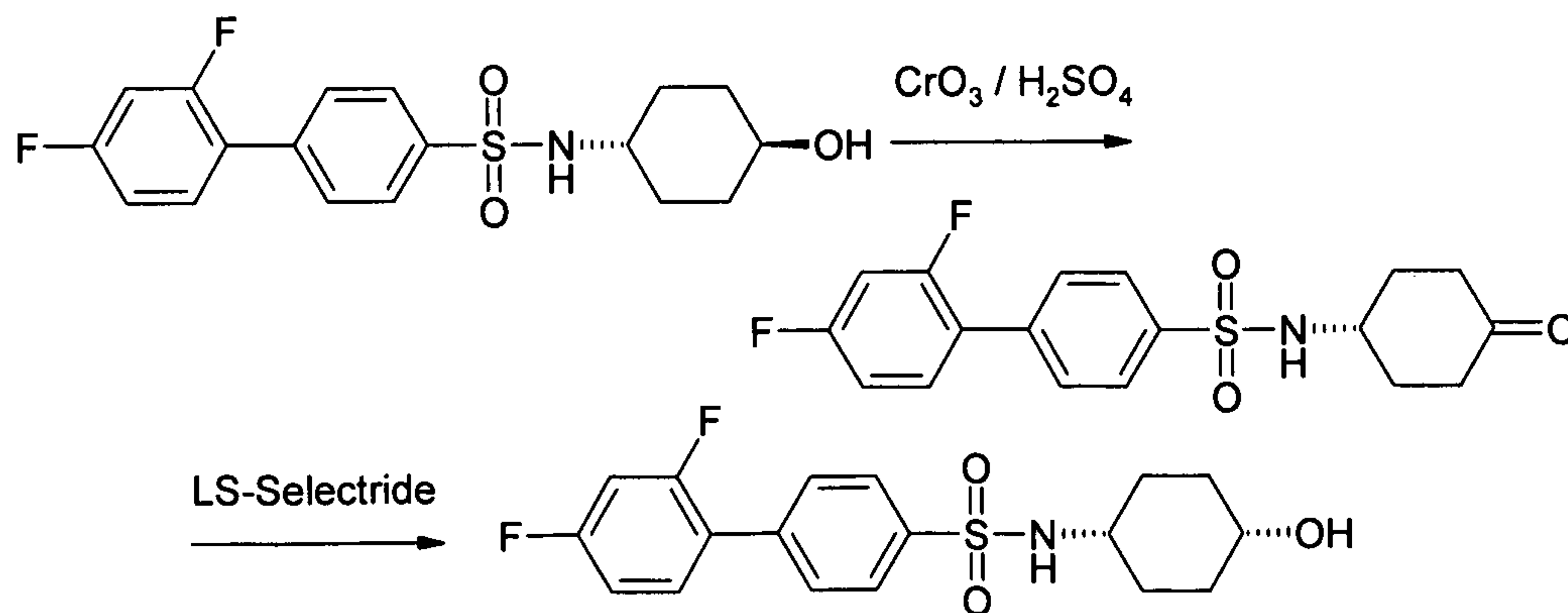
Scheme 14
