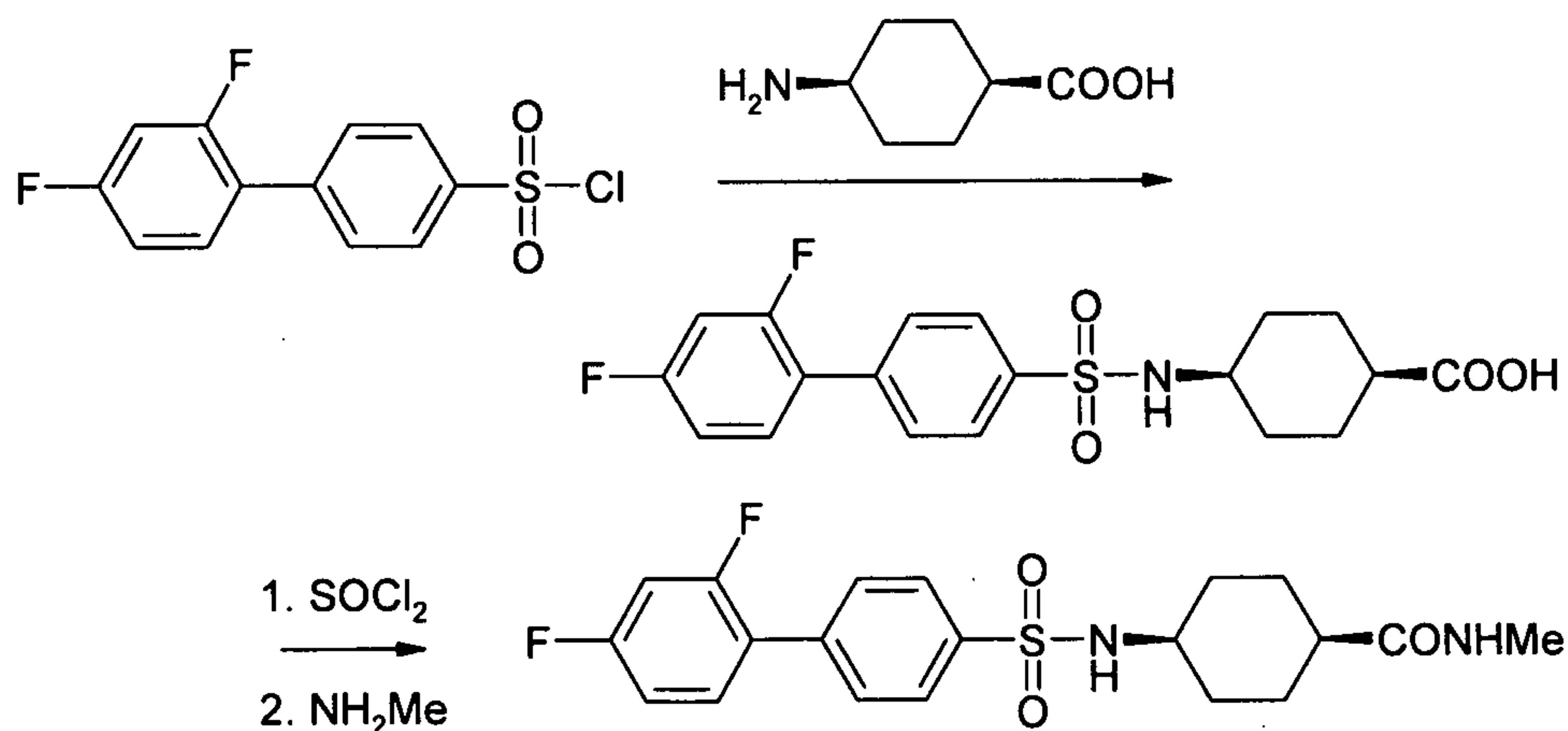
Scheme 8
