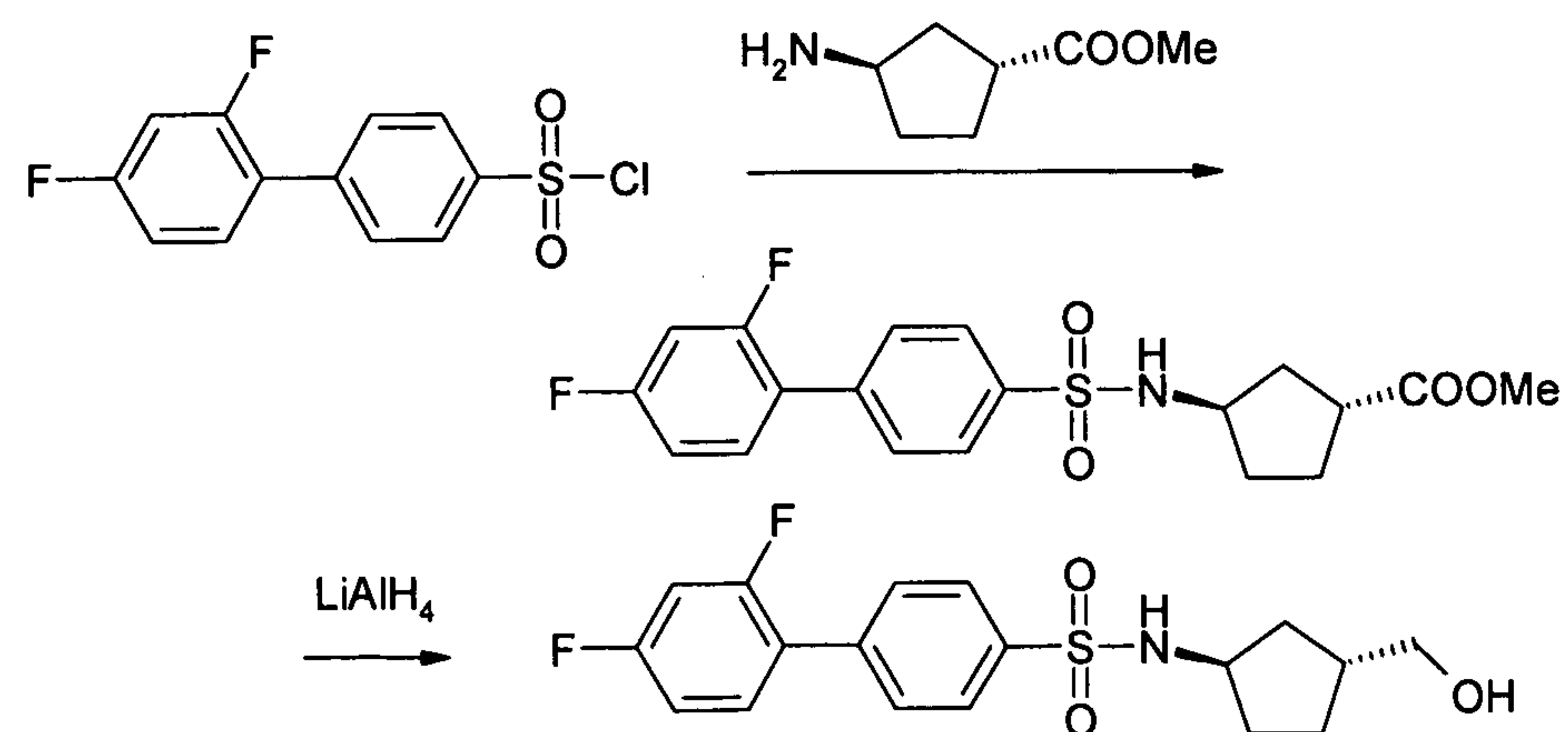
Scheme 6
