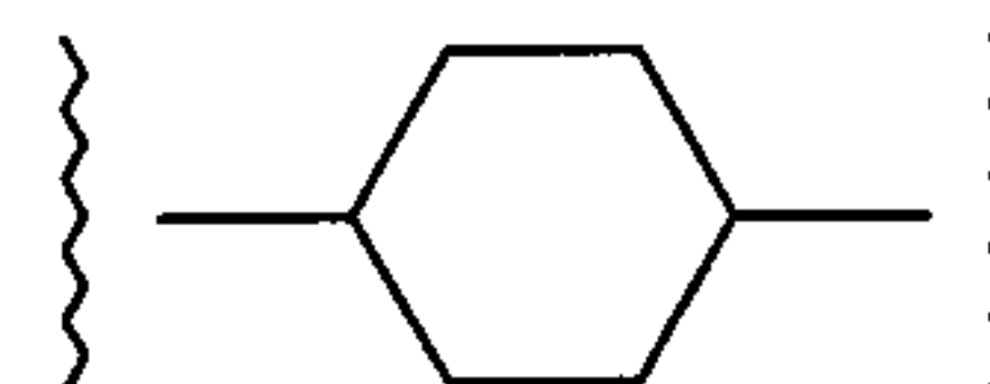
cyclohexane-1,4-di-yl
