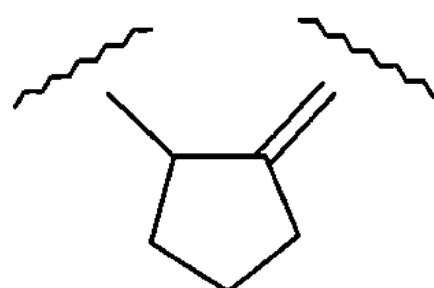
cyclopentane-1-yl-2-ylidene
