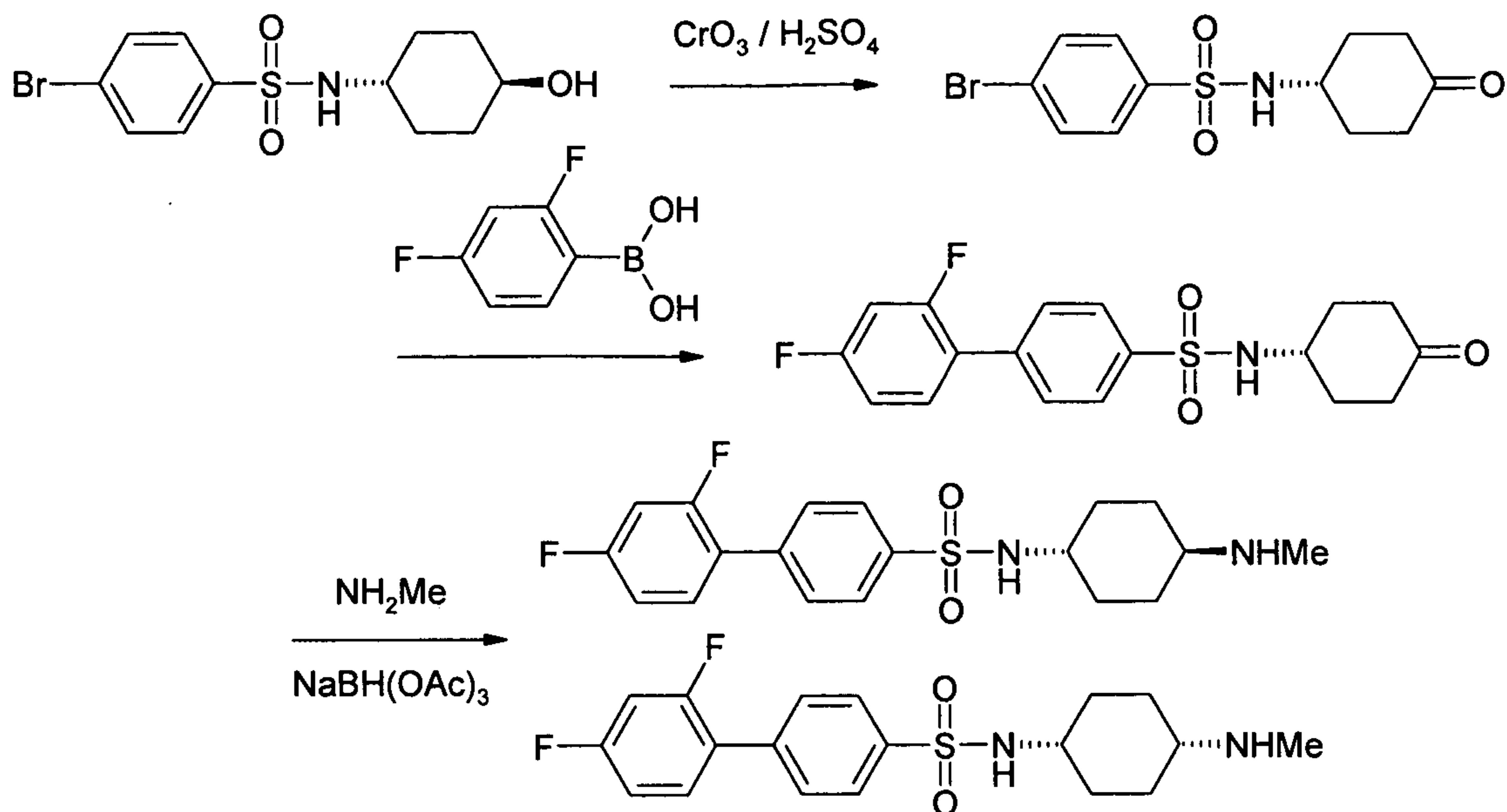
Scheme 11
