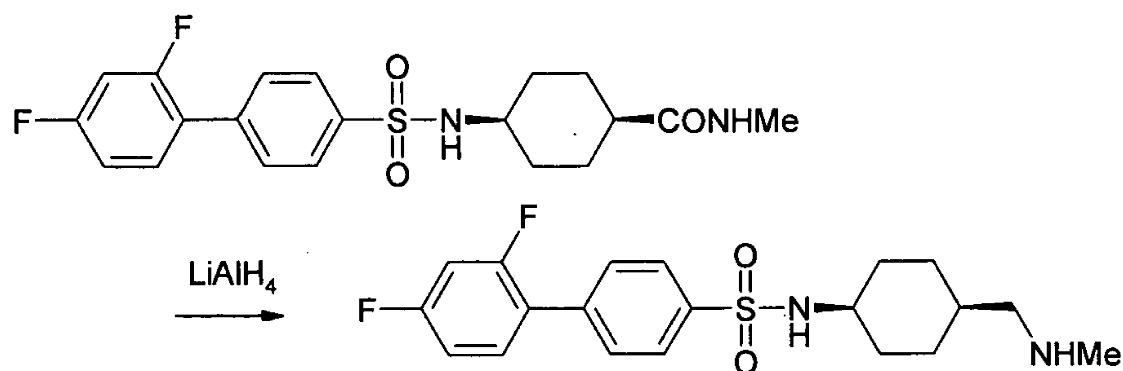
Scheme 9
