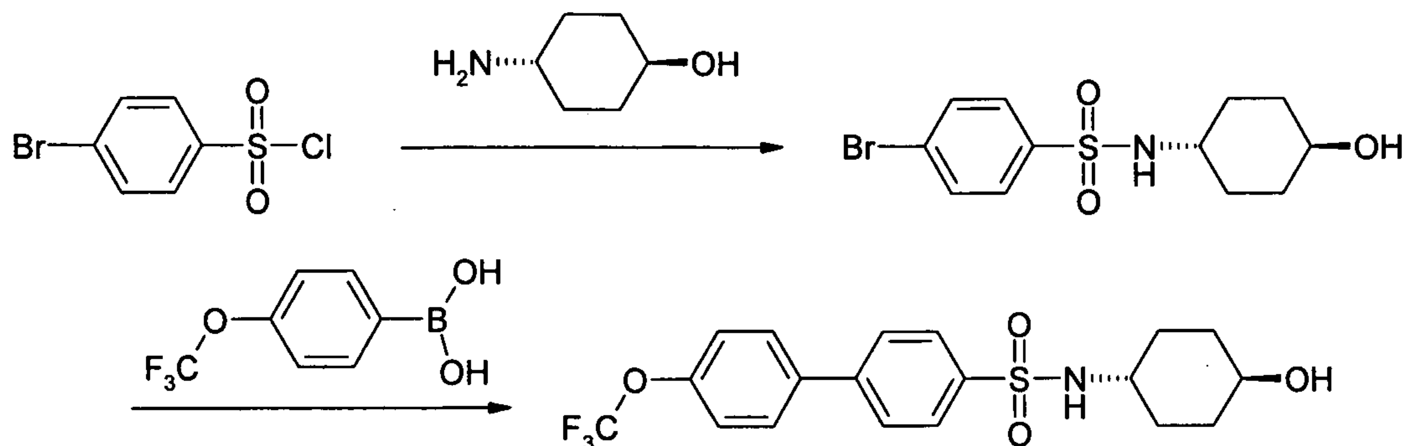
Scheme 2
