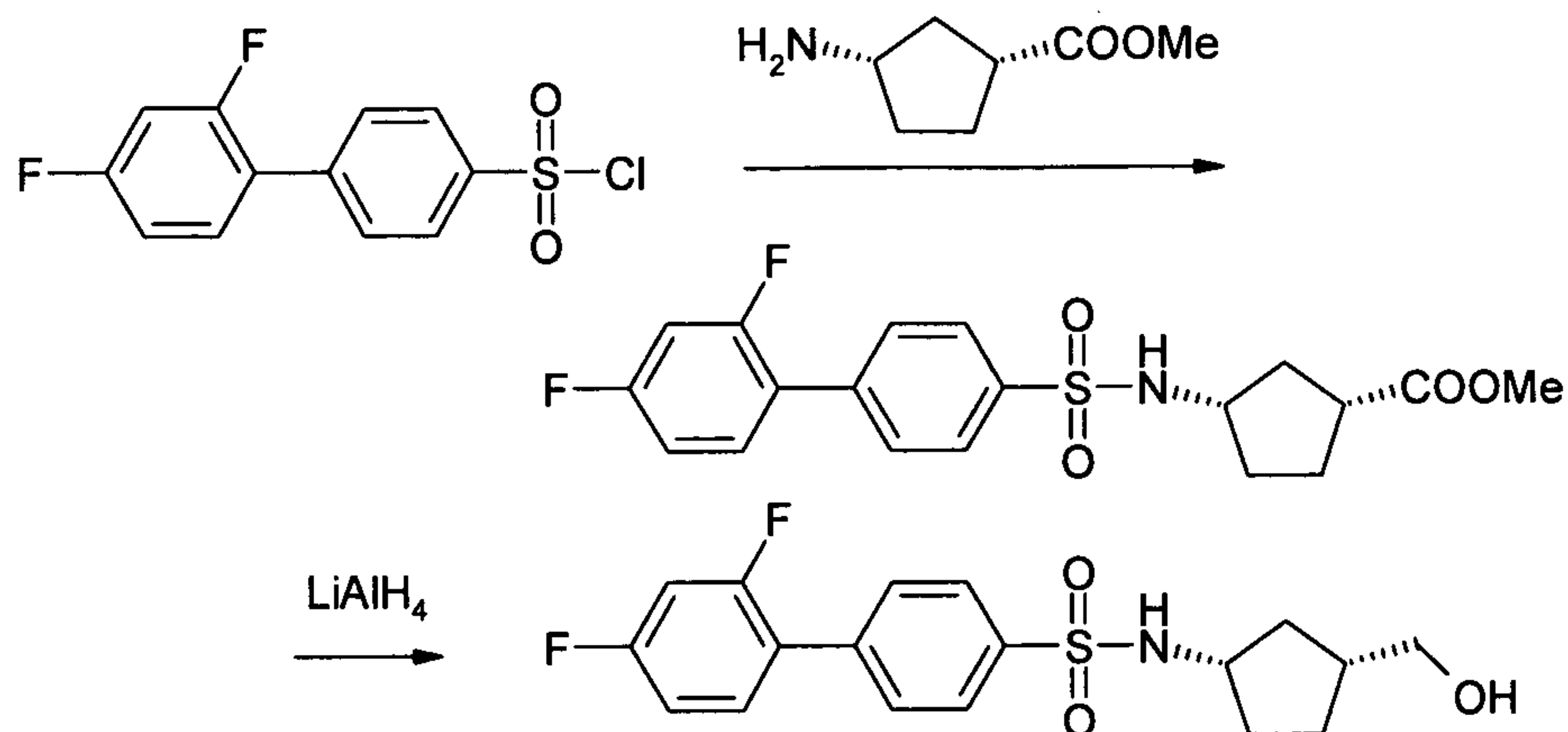
Scheme 4
