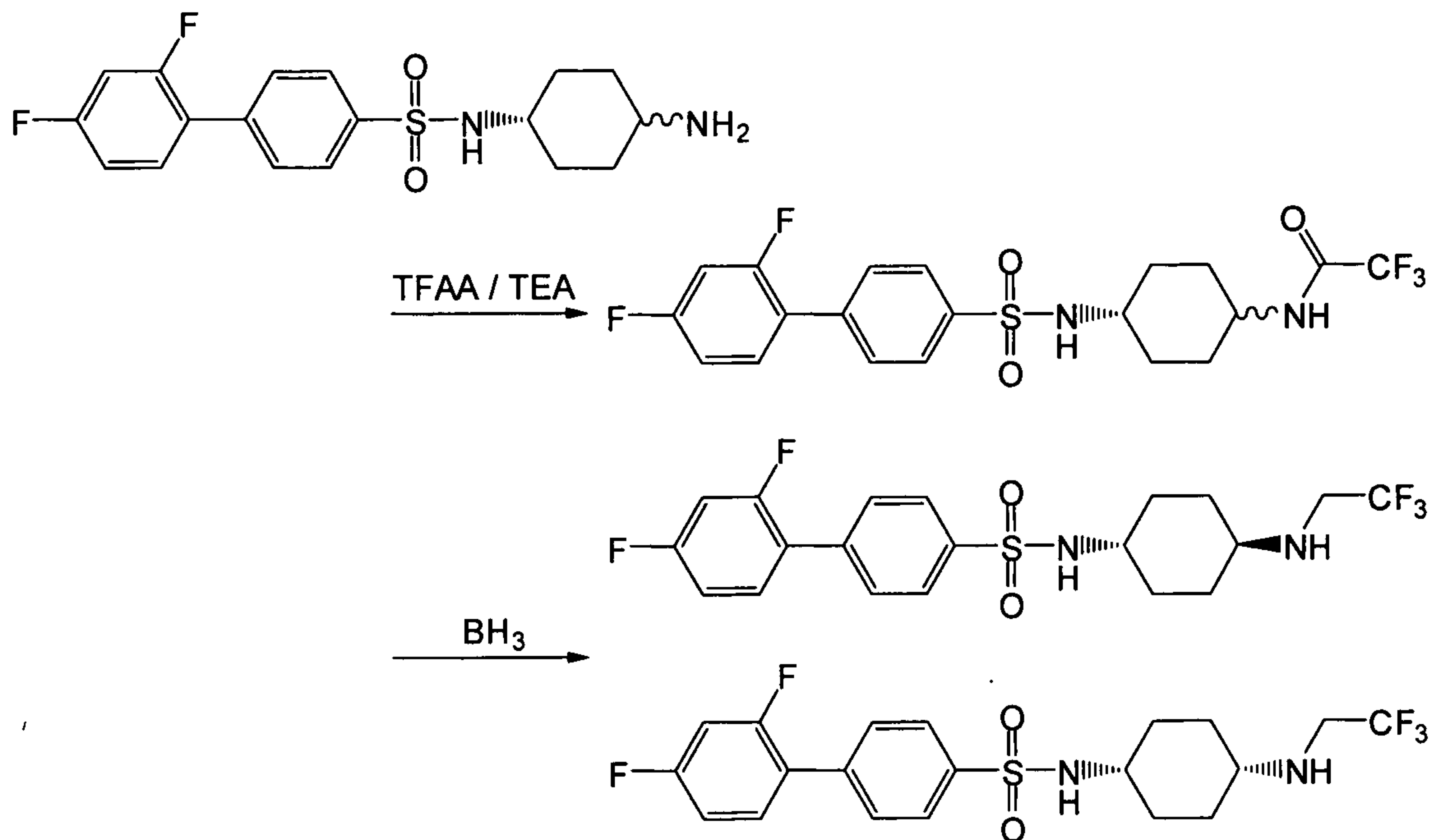
Scheme 13
