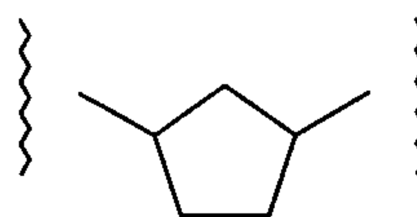
cyclopentane-1,3-di-yl
