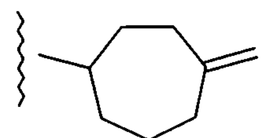
cycloheptane-1-yl-4-ylidene
