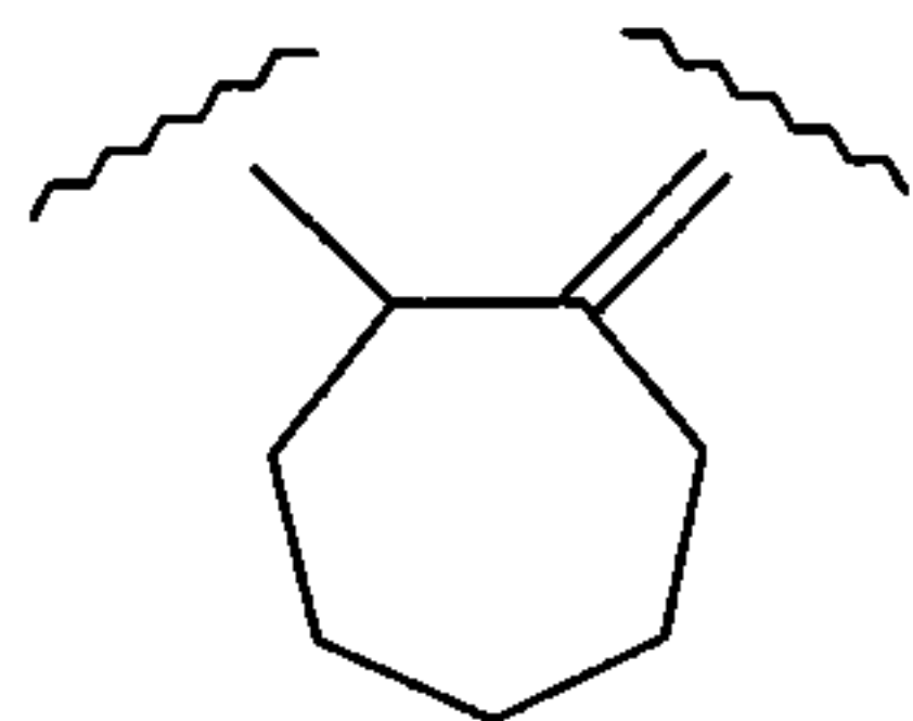
cycloheptane-1-yl-2-ylidene
