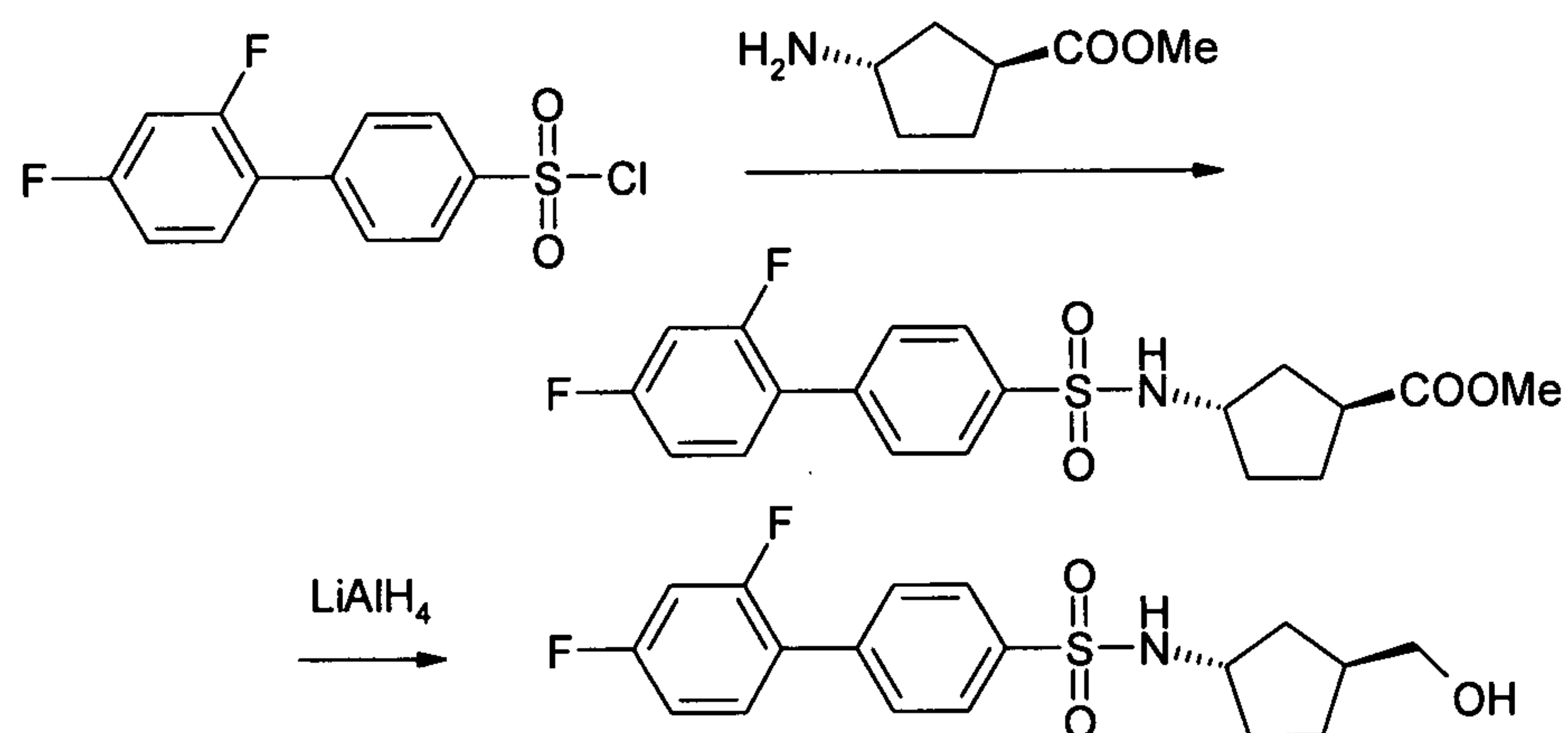
Scheme 5
