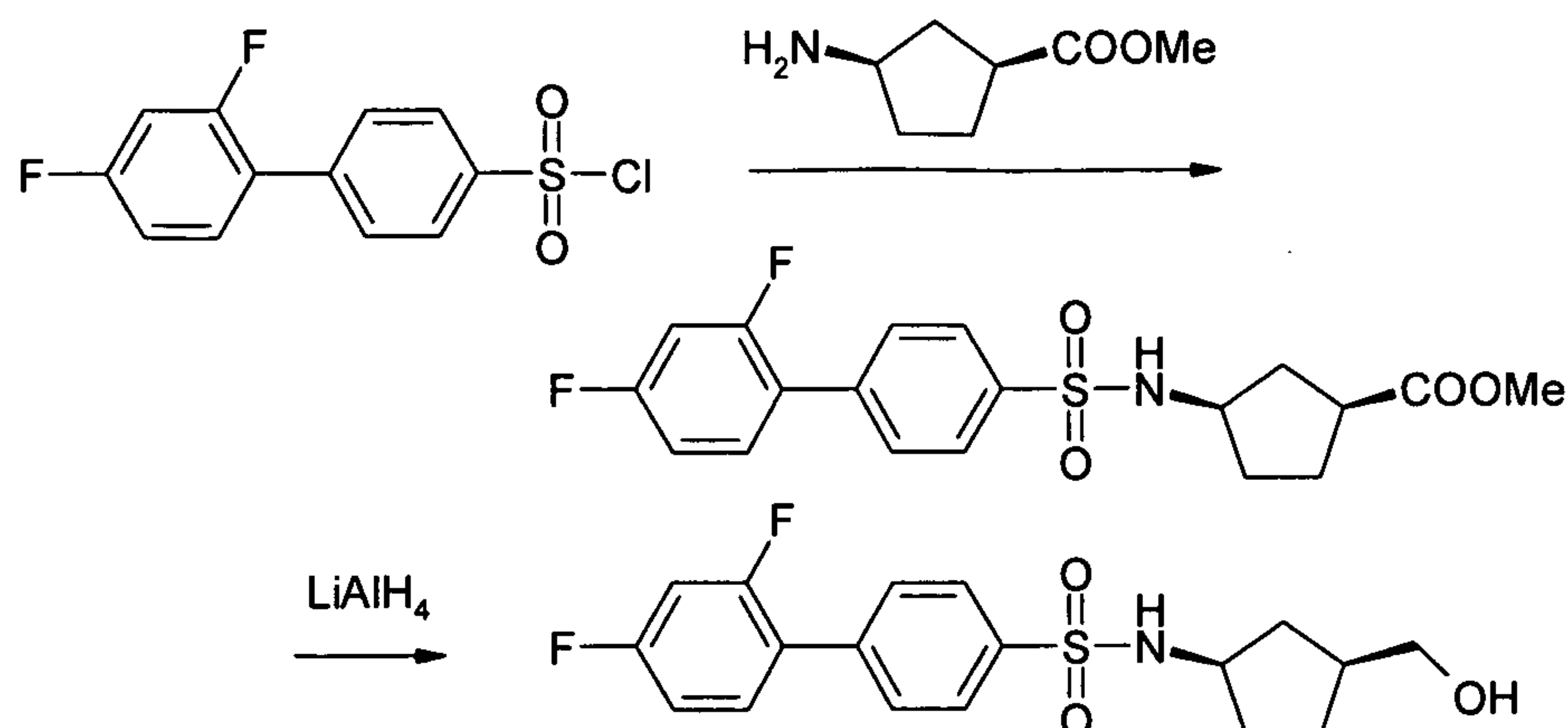
Scheme 7
