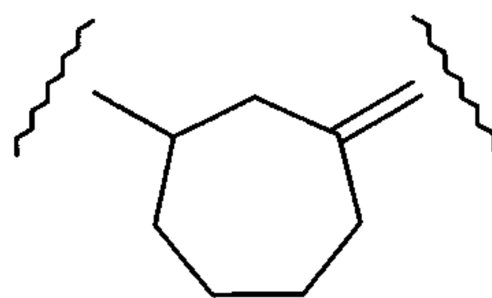
cycloheptane-1-yl-3-ylidene
