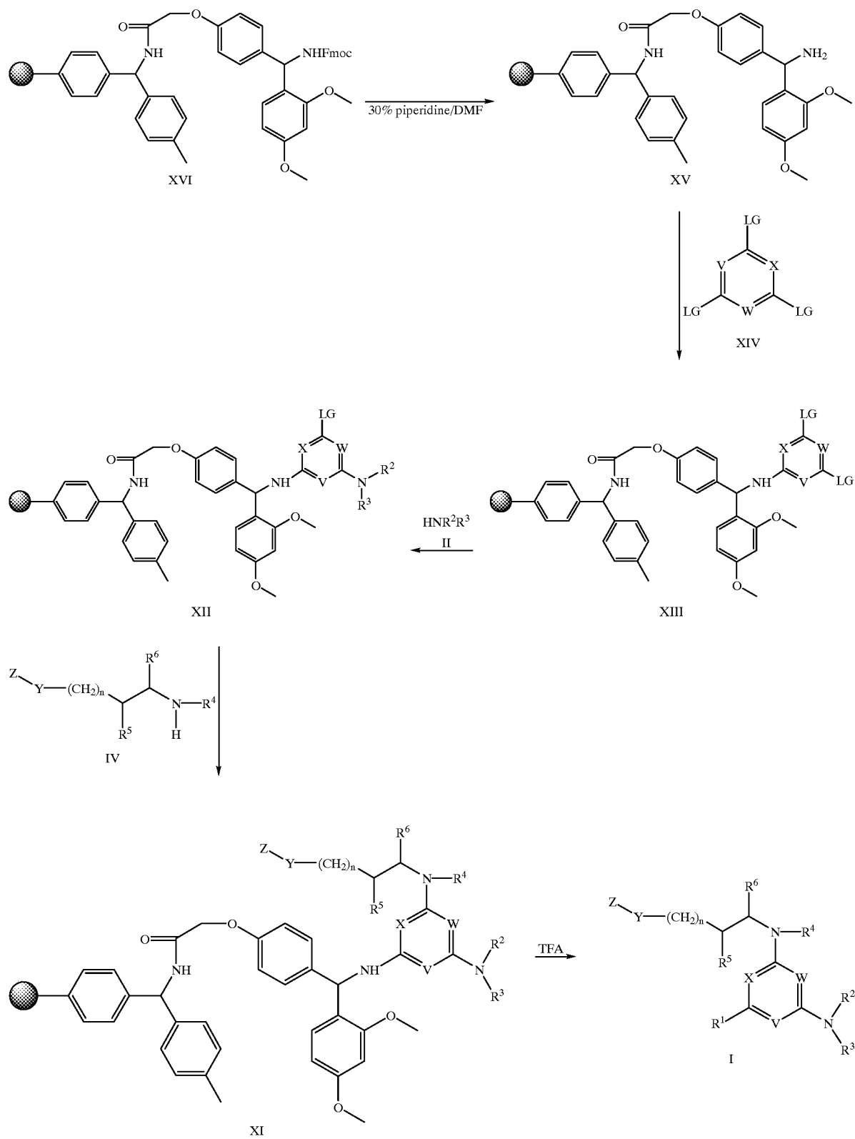
Scheme 2
