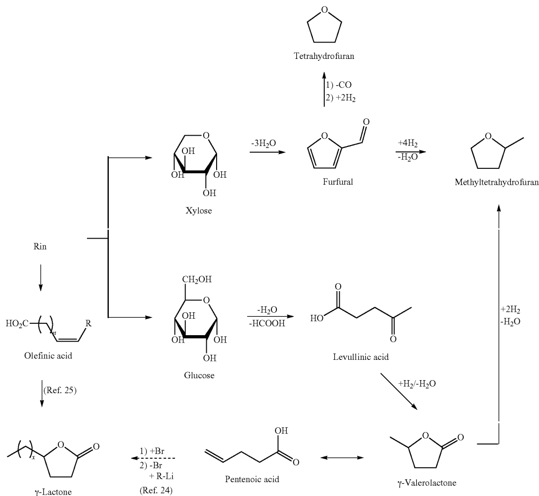
Reaction Scheme 2
