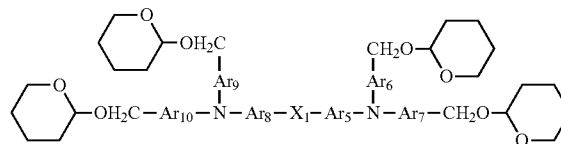
Chemical Structure 11
