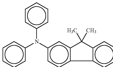
Chemical Structure 1
