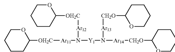
Chemical Structure 11
