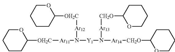
Chemical Structure 11
