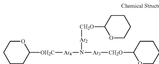
Chemical Structure 9
