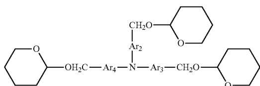
Chemical Structure 9
