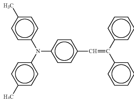
Chemical Structure 18
