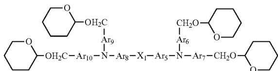
Chemical Structure 10
