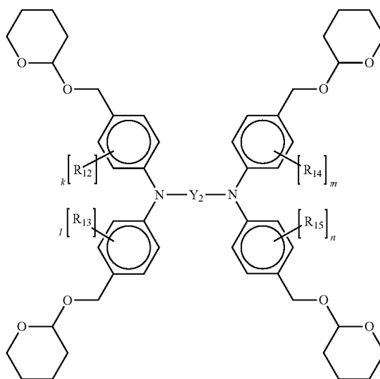
Chemical Structure 14
