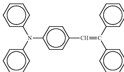
Chemical Structure 7
