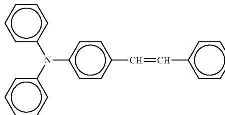
Chemical Structure 6
