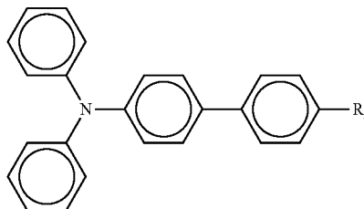
Chemical Structure 4
