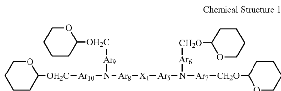
Chemical Structure 10
