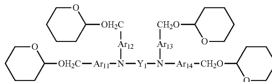
Chemical Structure 11
