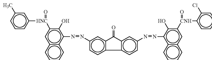
Chemical Structure 19
