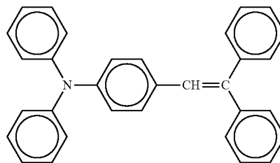
Chemical Structure 17
