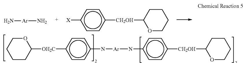
Chemical Reaction 5
