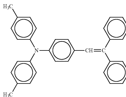
Chemical Structure 18
