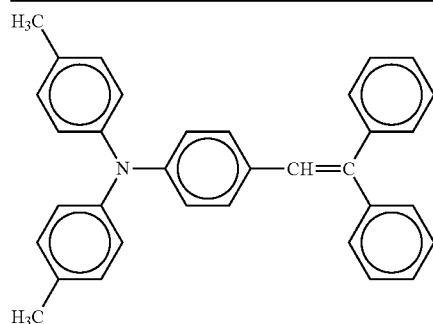
Chemical Structure 18
