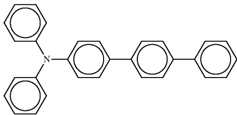
Chemical Structure 8
