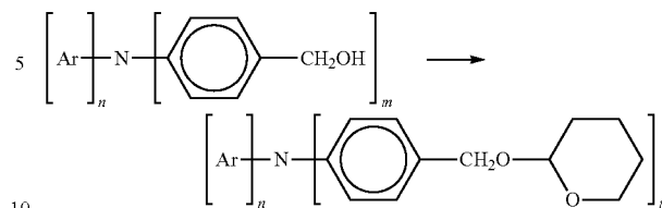
Chemical Reaction 3
