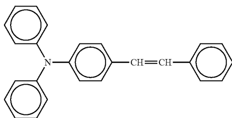
Chemical Structure 6
