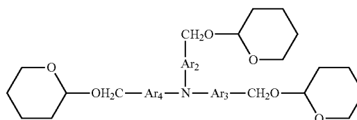
Chemical Structure 10
