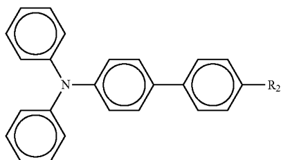
Chemical Structure 4
