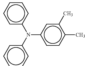
Chemical Structures
