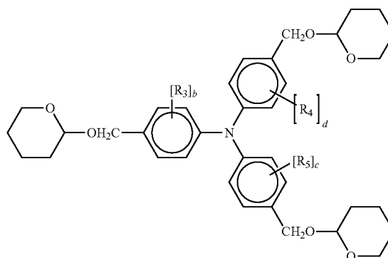
Chemical Structure 12
