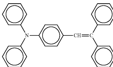
Chemical Structure 7
