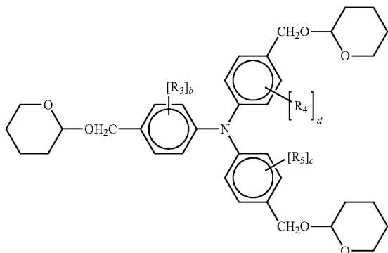
Chemical Structure 12
