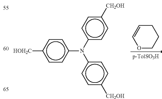
Chemical Reaction 8
