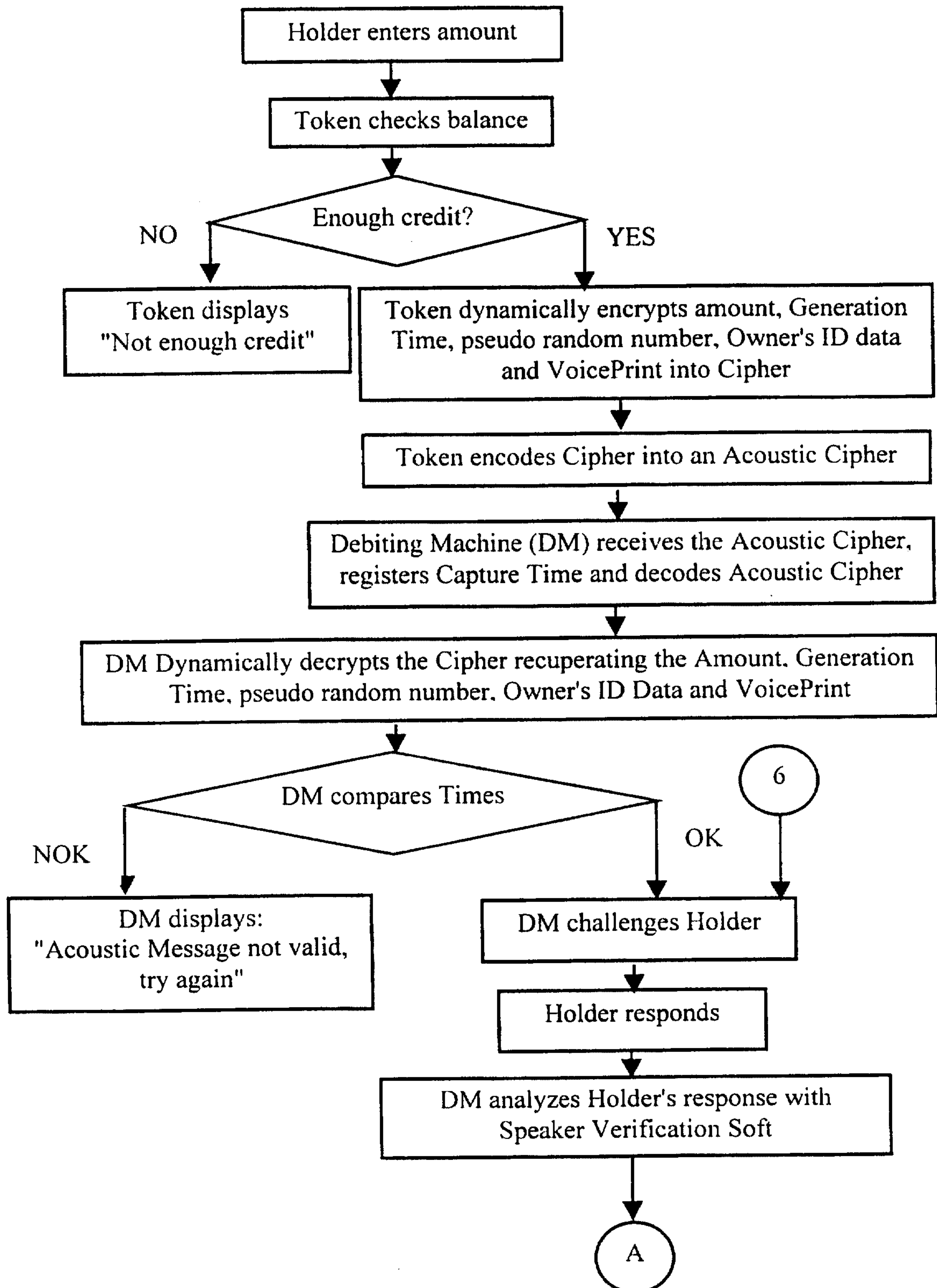
FIGURE 15 Acoustic Traveler's Check Flow Diagram, With Confirmation Number
