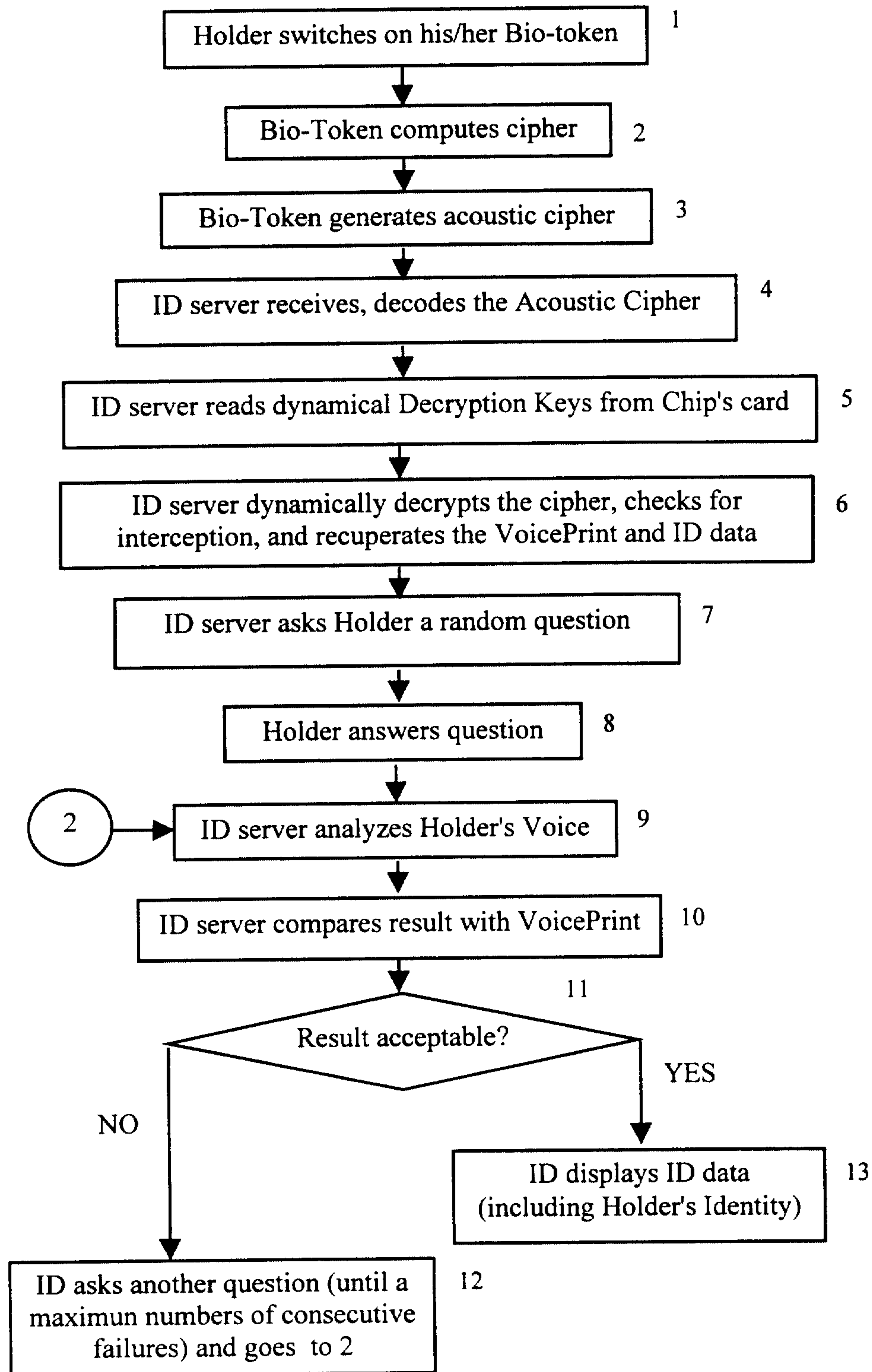
FIGURE 10 Identification Flow Case 1a
