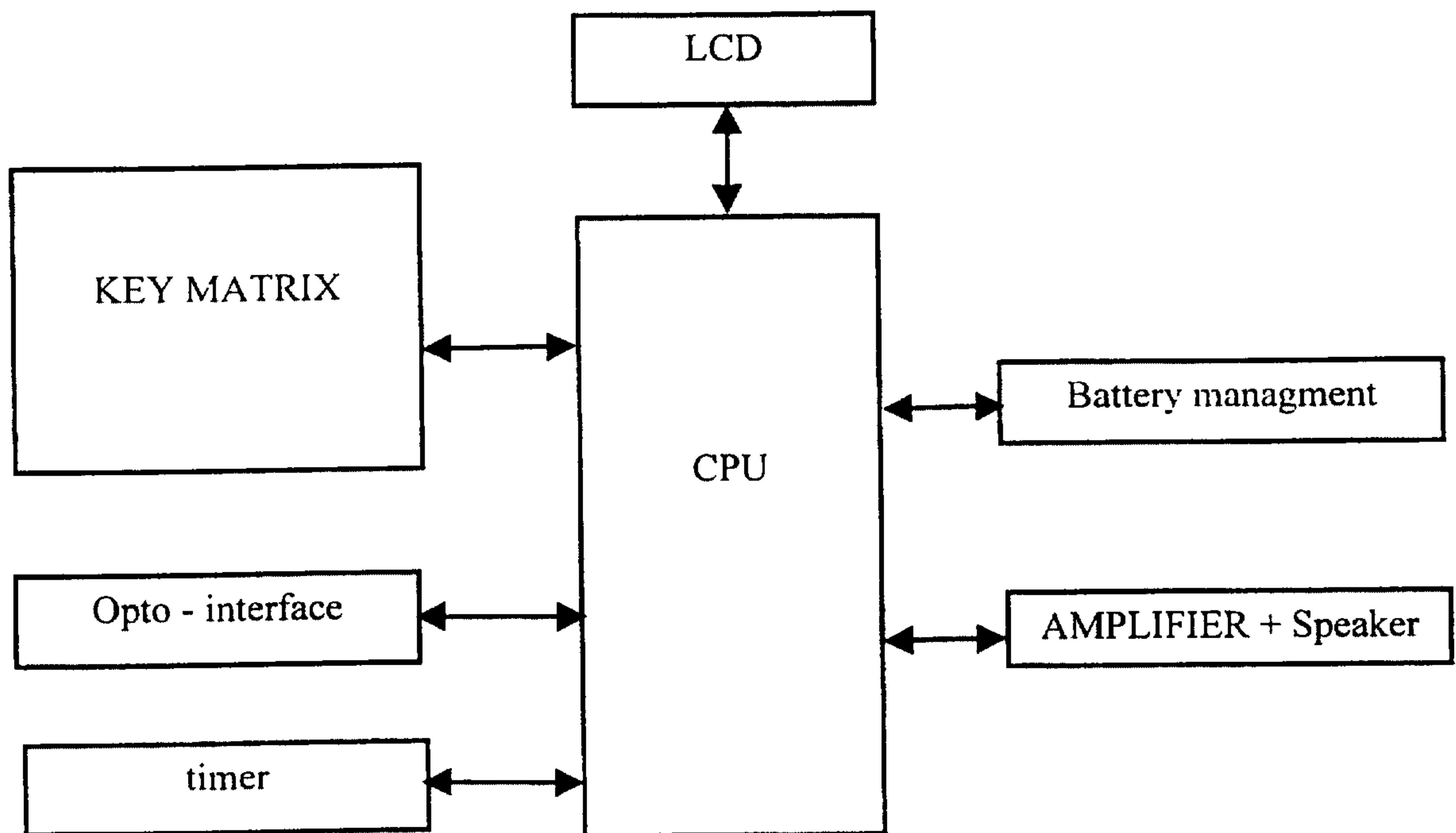
FIGURE 14 Bio-Token/ROV Bio-Token Block Description
