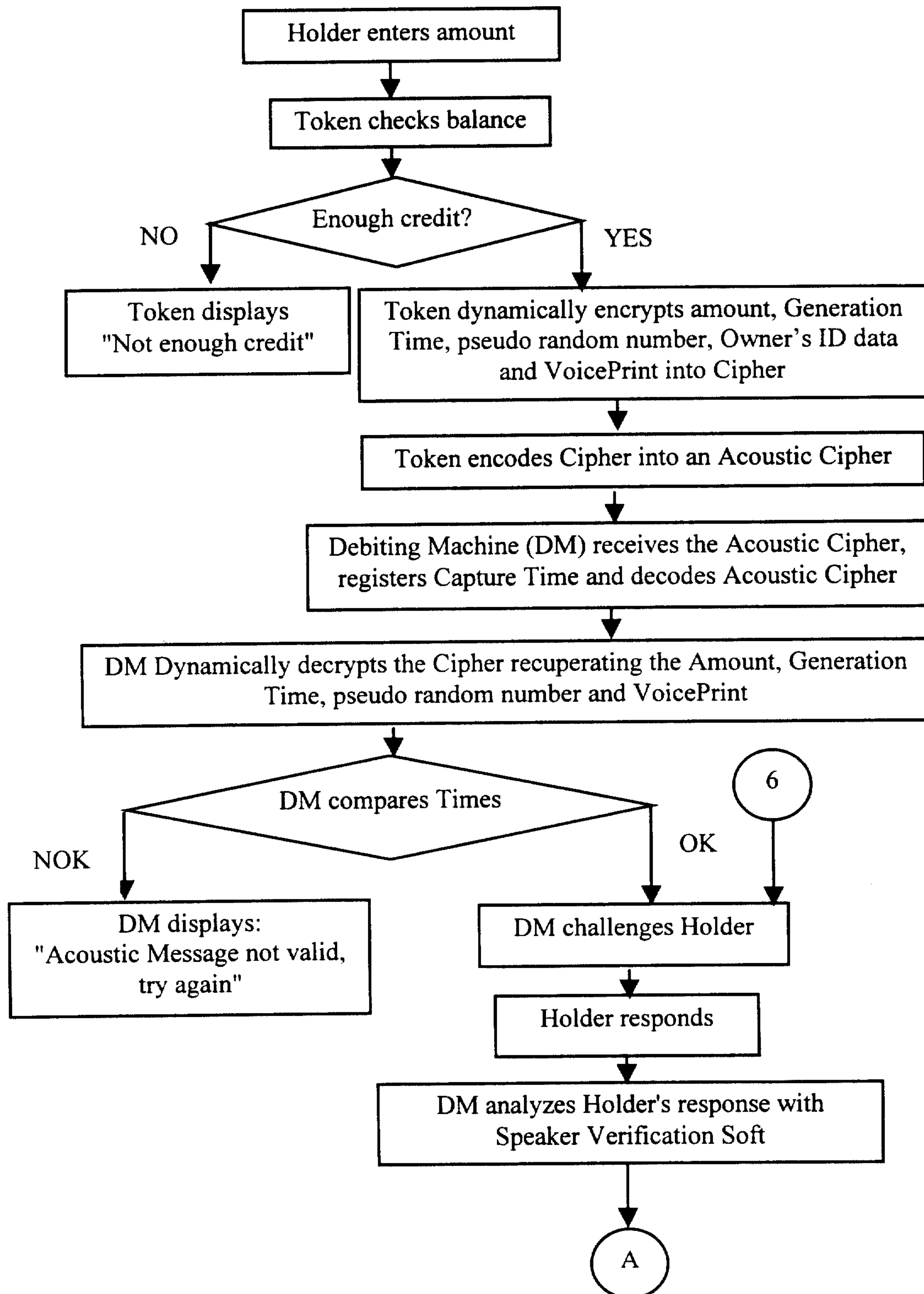
FIGURE 16 Debit Card Flow Diagram, With Confirmation Number
