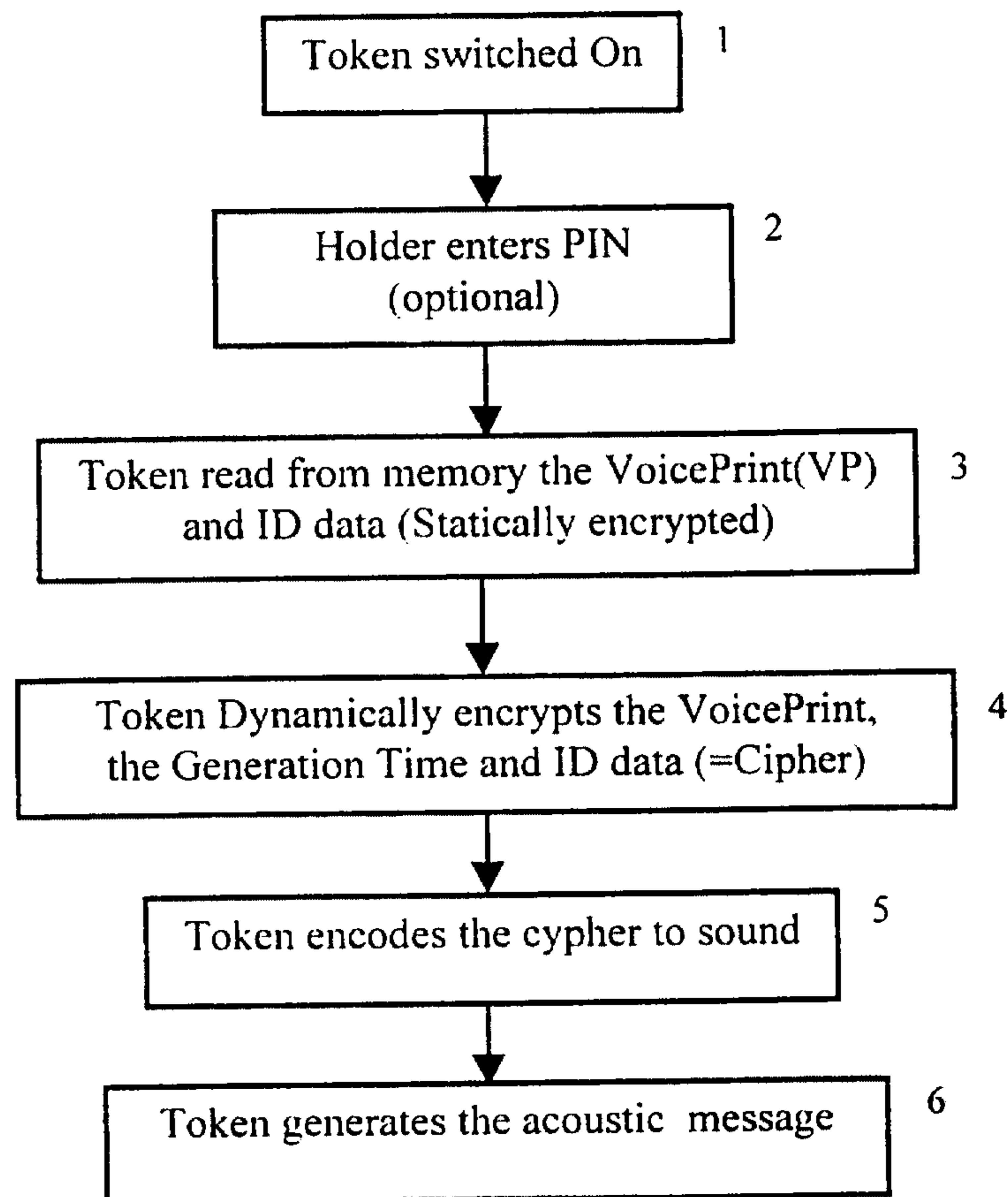
FIGURE 4 Token Methodology Case 2
