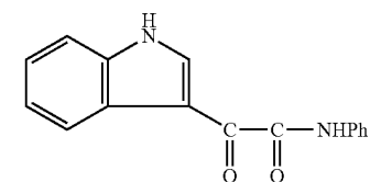
1H-Indole-3-acetamide, α-oxo-N-phenyl-
