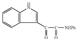
1H-Indole-3-acetamide, α-oxo-N-phenyl-
