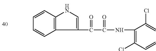
1H-Indole-3-acetamide, N-(2,6-dichlorophenyl)-α-oxo-
