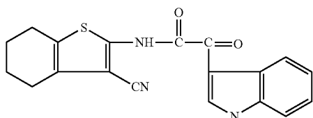
1H-Indole-3-acetamide, N-(3-cyano-4,5,6,7-tetrahydrobenzo[b]thien-2-yl)-α-oxo-
