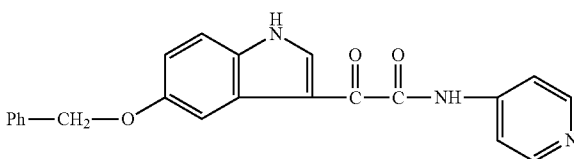
Indole-3-glyoxylamide, 5-(benzyloxy)-N-4-pyridyl-
