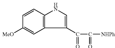
Indole-3-glyoxylanilide, 5-methoxy-
