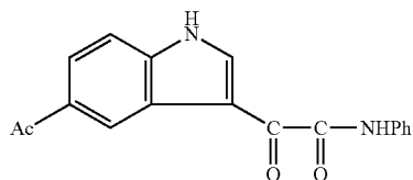
1H-Indole-3-acetamide, 5-acetyl-α-oxo-N-phenyl-
