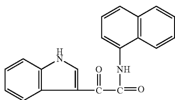
1H-Indole-3-acetamide, N-1-naphthalenyl-α-oxo-
