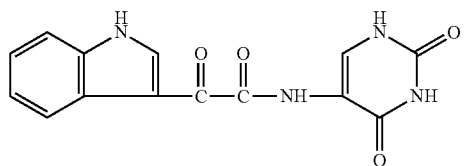
1H-Indole-3-acetamide, α-oxo-N-(1,2,3,4-tetrahydro-2,4-dioxo-5-pyrimidinyl)-
