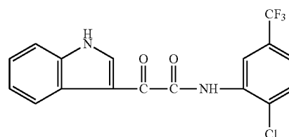
1H-Indole-3-acetamide, N-[2-chloro-5-(trifluoromethyl)phenyl]-α-oxo-
