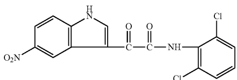
1H-Indole-3-acetamide, N-(2,6-dichlorophenyl)-5-nitro-α-oxo-
