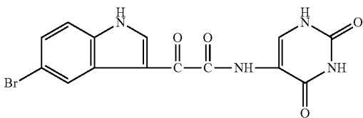
1H-Indole-3-acetamide, 5-bromo-α-oxo-N-(1,2,3,4-tetrahydro-2,4-dioxo-5-pyrimidinyl)-
