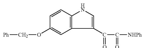
Indole-3-glyoxylanilide, 5-(benzyloxy)-
