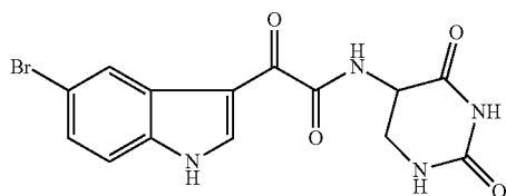
2-(5-bromo-1H-indol-3-yl)-N-(2,4-dioxo-1,2,3,4-tetrahydropyrimidin-5-yl)-2-oxo-acetamide
