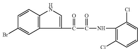
1H-Indole-3-acetamide, 5-bromo-N-(2,6-dichlorophenyl)-α-oxo-
