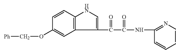
Indole-3-glyoxylanilide, 5-(benzyloxy)-N-2-pyridyl-
