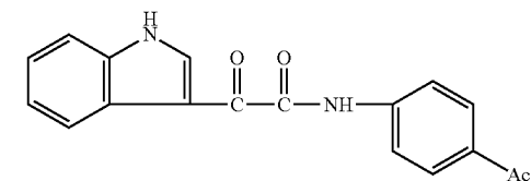
Indole-3-glyoxylanilide, 4'-acetyl-
