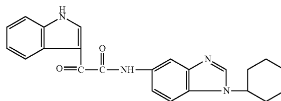
1H-Indole-3-acetamide, N-(1-cyclohexyl-1H-benzimidazol-5-yl)-α-oxo-
