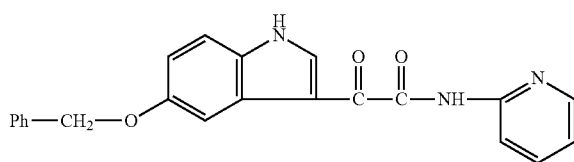
Indole-3-glyoxylamide, 5-(benzyloxy)-N-3-pyridyl-
