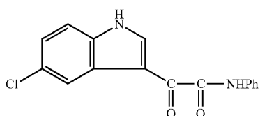
1H-Indole-3-acetamide, 5-chloro-α-oxo-N-phenyl-
