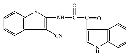
1H-Indole-3-acetamide, N-[3-cyanobenzo(b)thien-2-yl]-α-oxo-
