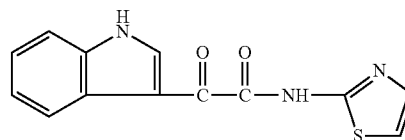
1H-Indole-3-acetamide, α-oxo-N-2-thioxolyl-
