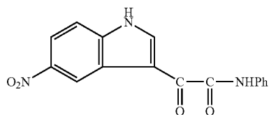
1H-Indole-3-acetamide, 5-nitro-α-oxo-N-phenyl-
