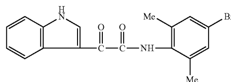
1H-Indole-3-acetamide, N-(4-bromo-2,5-dimethylphenyl)-α-oxo-
