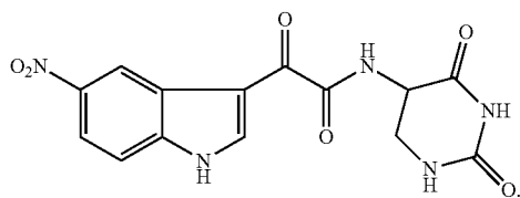
N-(2,4-dioxo-1,2,3,4-tetrahydropyrimidin-5-yl)-2-(5-nitro-1H-indol-3-yl)-2-oxo-acetamide
