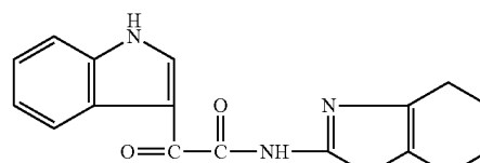
1H-Indole-3-acetamide, α-oxo-N-(4,5,6,7-tetrahydro-2-benzothiazolyl)-
