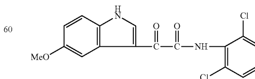
1H-Indole-3-acetamide, N-(2,6-dichlorophenyl)-5-methoxy-α-oxo-
