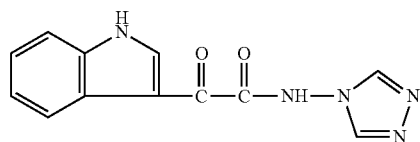
1H-Indole-3-acetamide, α-oxo-N-4H-1,2,4-triazol-4-yl-
