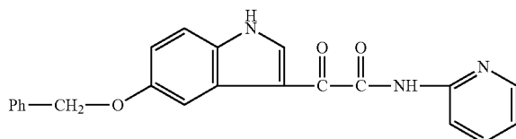
Indole-3-glyoxylamide, 5-(benzyloxy)-N-2-pyridyl-
