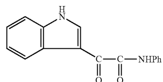
1H-Indole-3-acetamide, α-oxo-N-phenyl-
