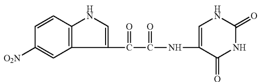
1H-Indole-3-acetamide, 5-nitro-α-oxo-N-(1,2,3,4-tetrahydro-2,4-dioxo-5-pyrimidinyl)-
