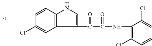
1H-Indole-3-acetamide, 5-chloro-N-(2,6-dichlorophenyl)-α-oxo-
