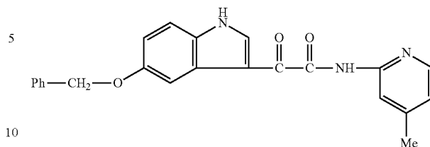
Indole-3-glyoxylanilide, 5-(benzyloxy)-N-(4-methyl-2-pyridyl)-
