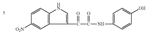
1H-Indole-3-acetamide, N-(4-hydroxyphenyl)-5-nitro-α-oxo-
