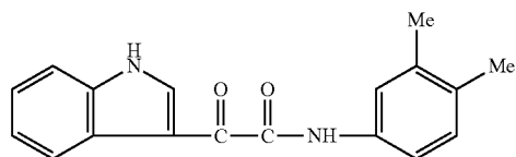
1H-Indole-3-acetamide, N-(3,4-dimethylphenyl)-α-oxo-
