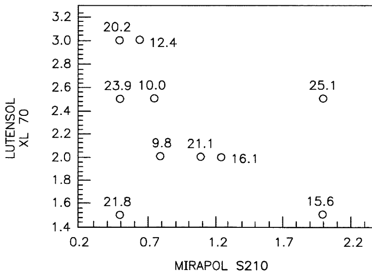
MEAN CONTACT ANGLE AFTER THIRTY RINSES
