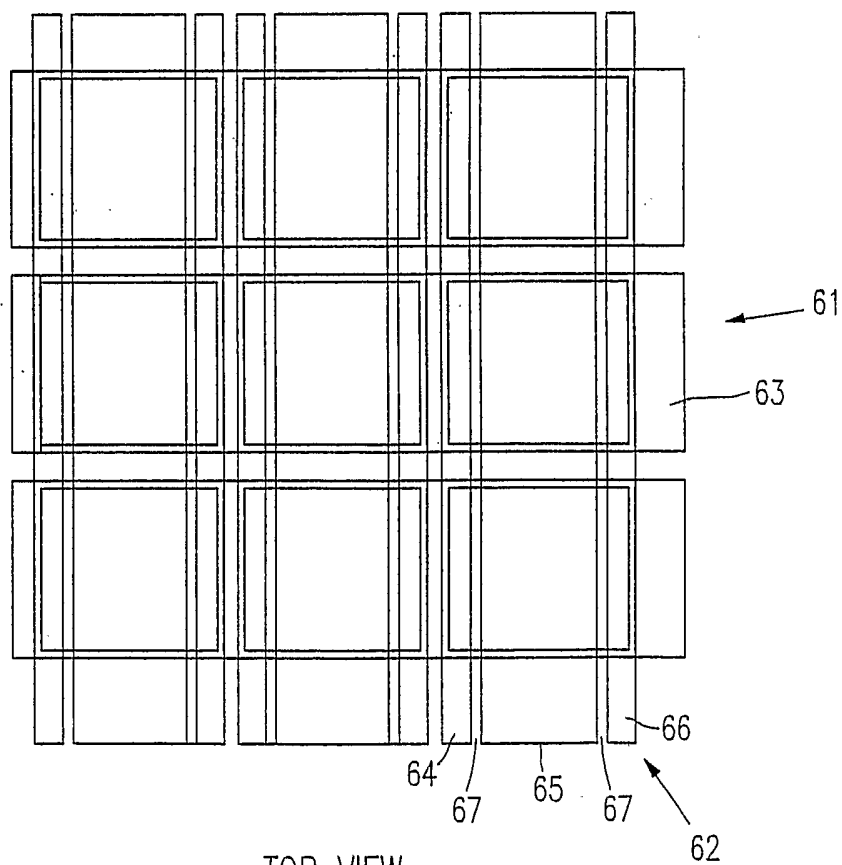
TOP VIEW FIG. 6B
