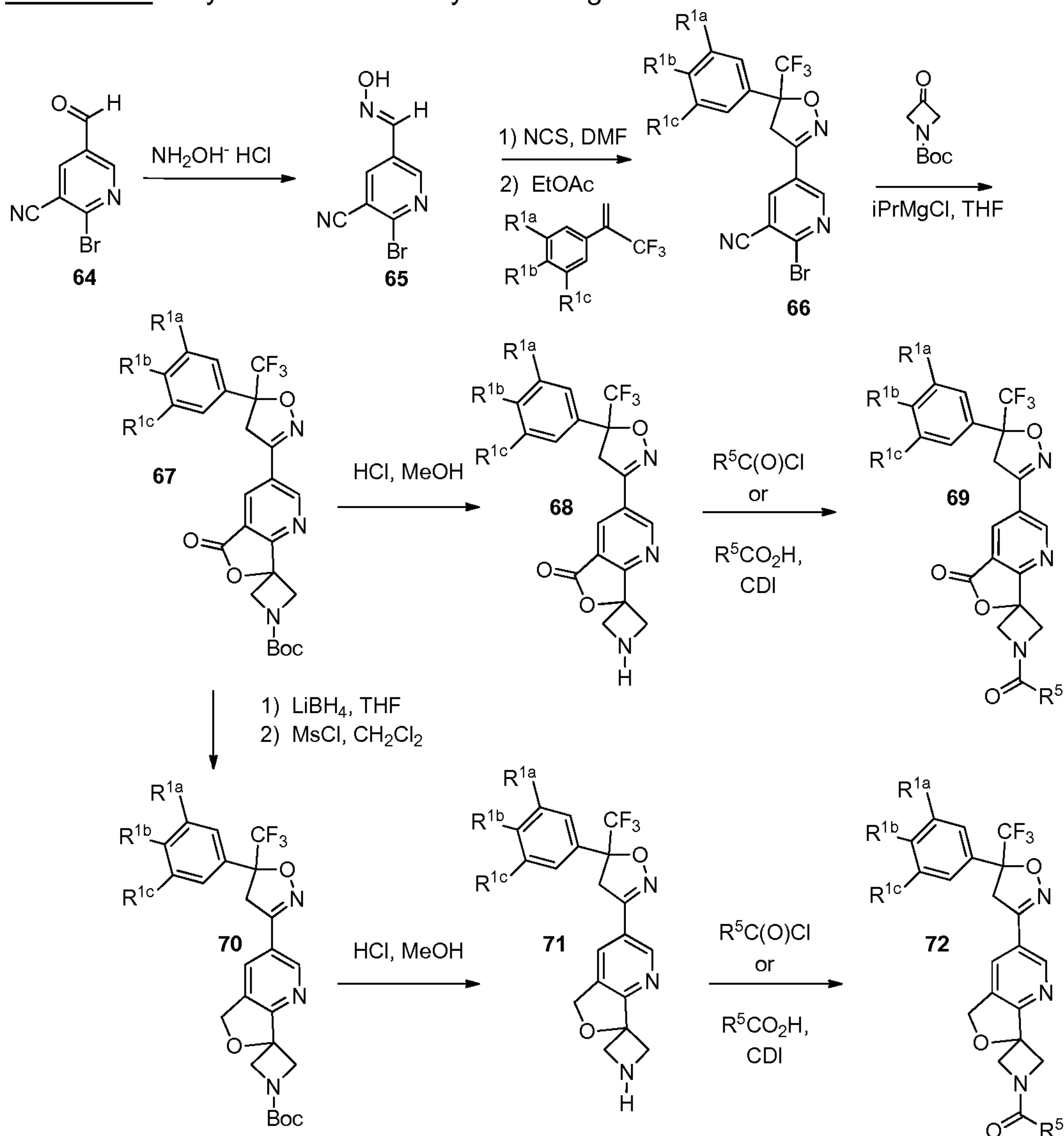
Scheme 17 – Synthesis of heterocyclic analogs
