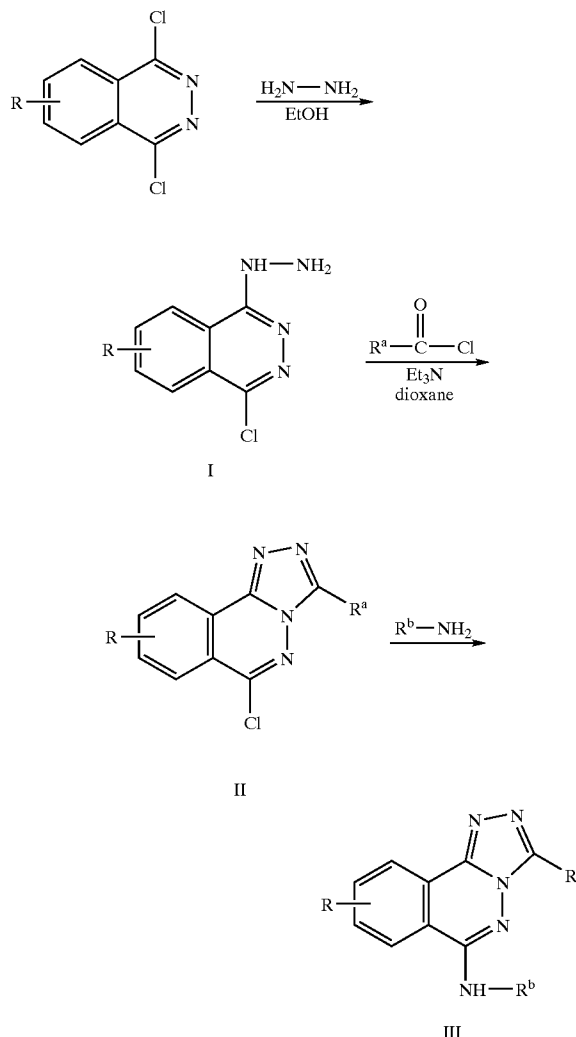
Reaction Scheme 1
