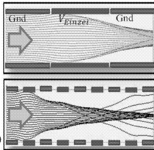
Fig. 2 Electron beam tracking simulations in Einzel focusing, for a) various V_{Einzel} for constant A/D=1 ; b) various Einzel A/D , constant V_{Einzel}=500V ; c) cascaded Einzel with same V_{Einzel} and total length.
