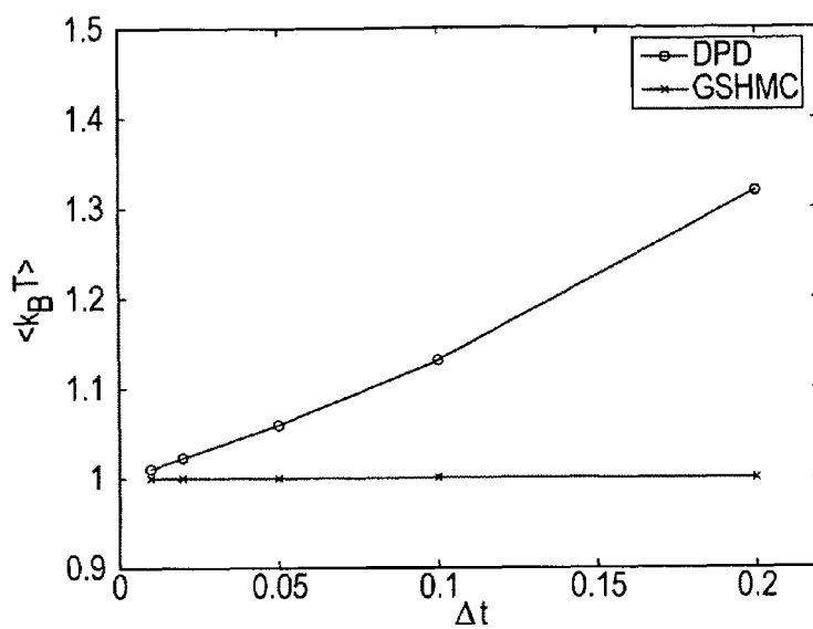
FIG. 5: Model A; Numerically Observed Temperature
