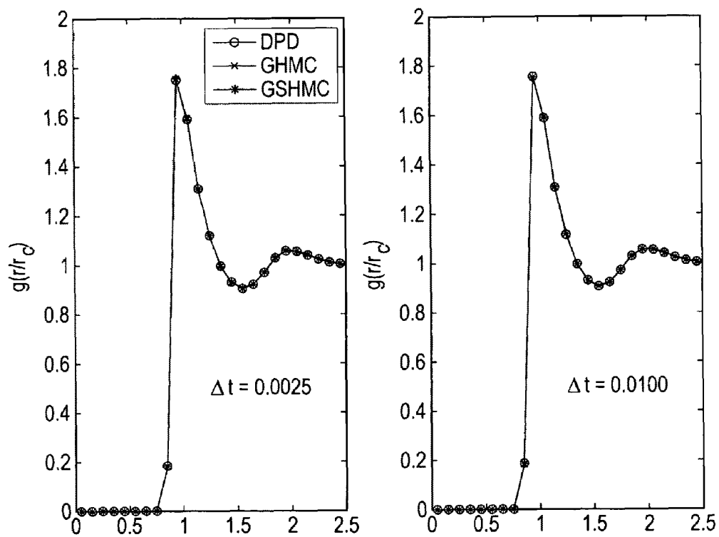
FIG. 6 Model C; Radial Distribution Function
