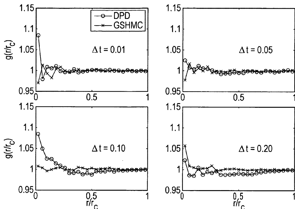
FIG. 3: Model A; Radial Distribution Function
