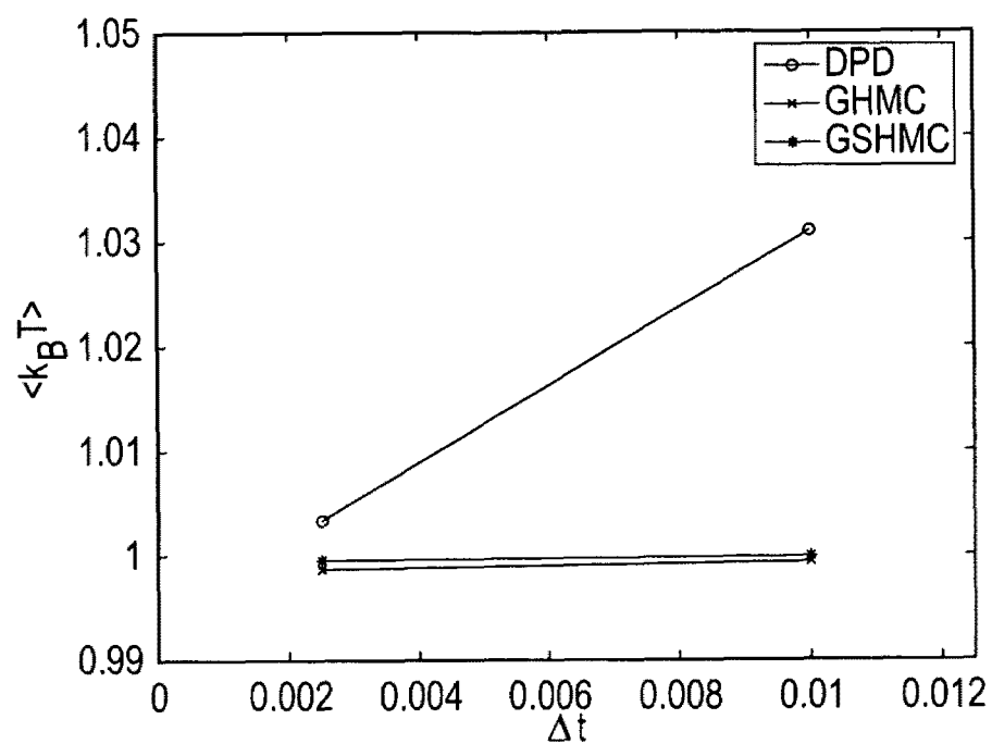
FIG. 7: Model C; Numerically Observed Temperature
