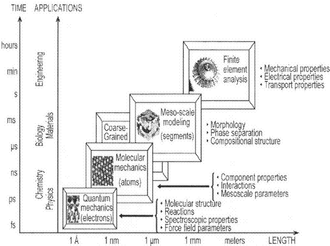
FIG. 1: Hierarchy of Scales
