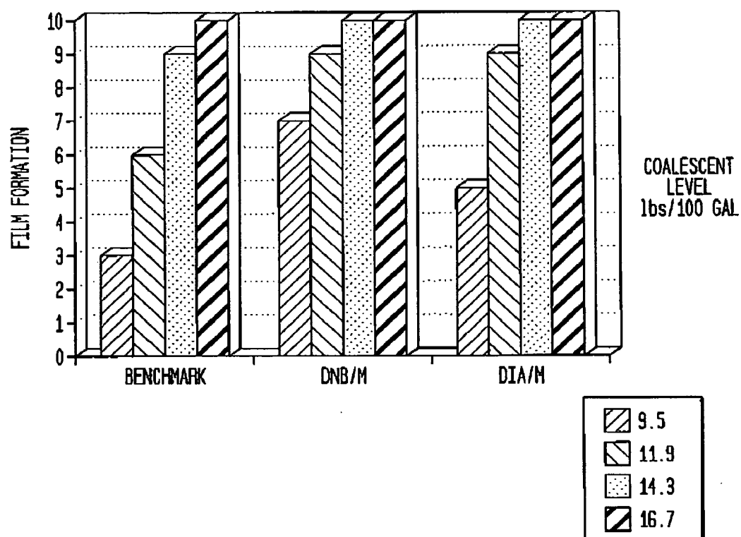
FIG. 8 LOW TEMPERATURE FILM FORMATION - SEMI-GLOSS PAINT
