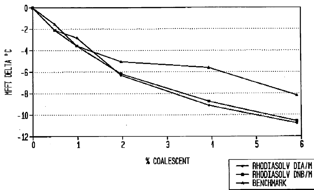
FIG. 7 MFFT RESULTS FOR VINYL-ACRYLIC RESIN
