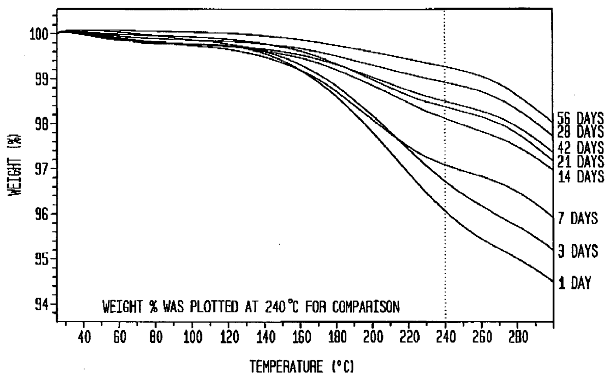
FIG. 9 RESIDUAL COALESCENTS IN DRIED PAINT FILM
