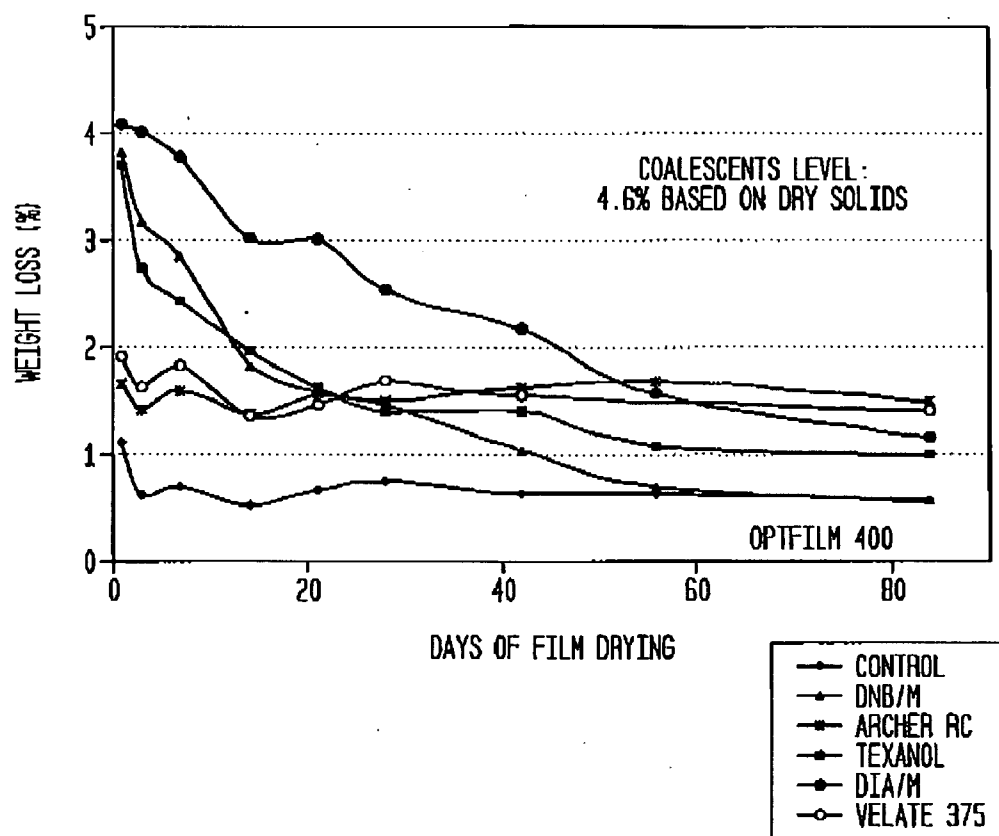
FIG. 10 RESIDUAL COALESCENT IN PAINT FILM - TGA ANALYSIS
