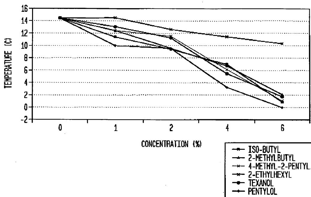
FIG. 2 EFFECT OF BRANCHED DIALKYL GLUTARATE ESTERS ON HFFT
