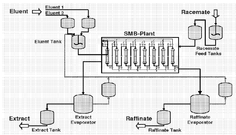
Figure 5: Example of a racemate separation:
