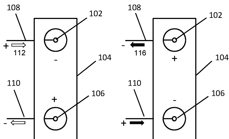
Positive Pulse
