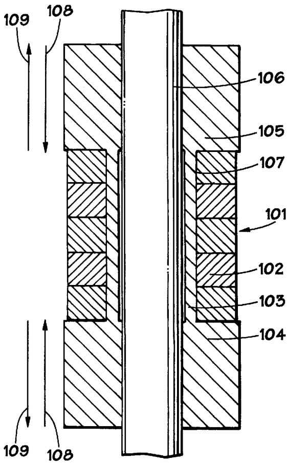
FIG. 1 (PRIOR ART)
