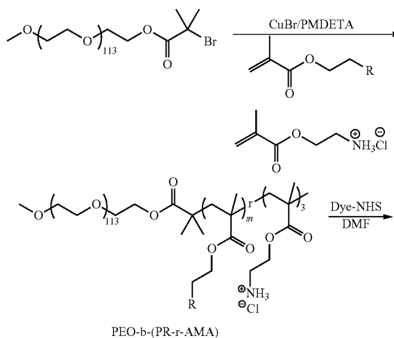
Scheme 1: Synthesis of Ionizable Segment
