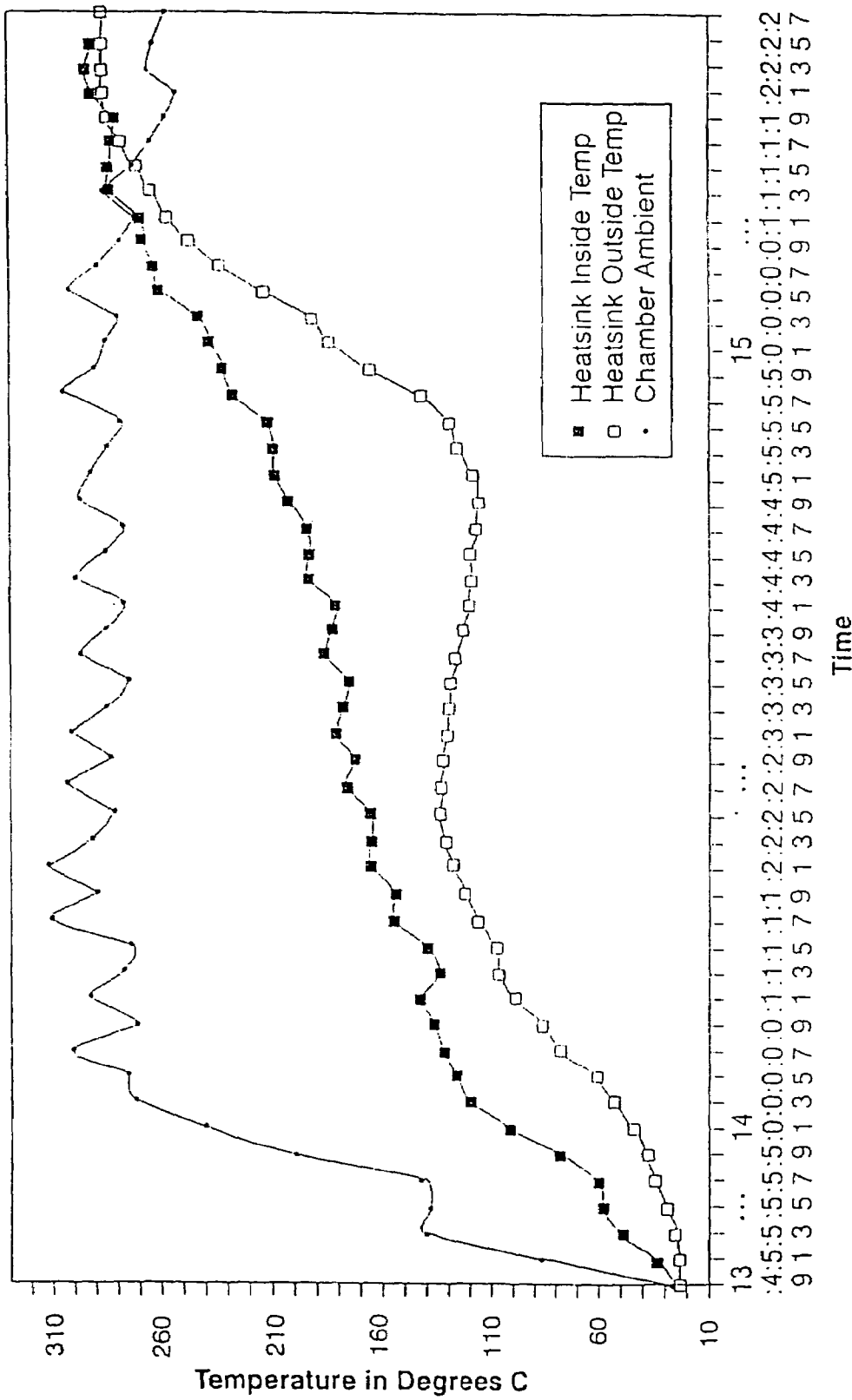
Test of Flight Recorder Heat Sink
