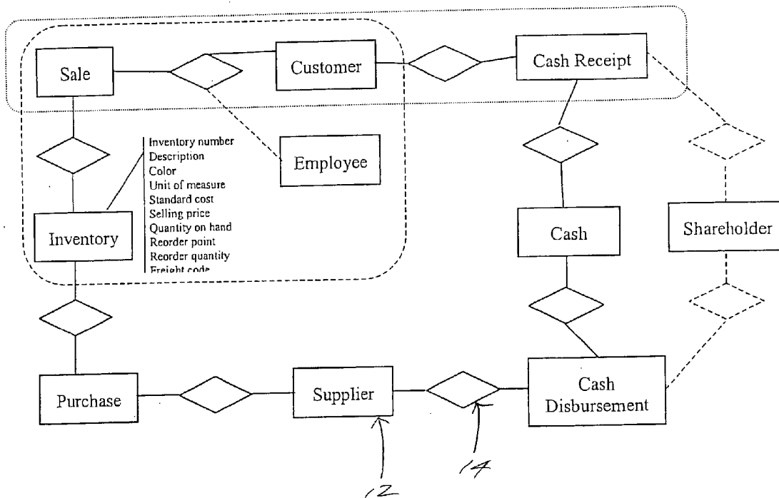
. An entity-relationship view of the sale and purchase events (under REA)
