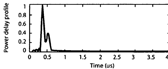
(c) Power delay profile
