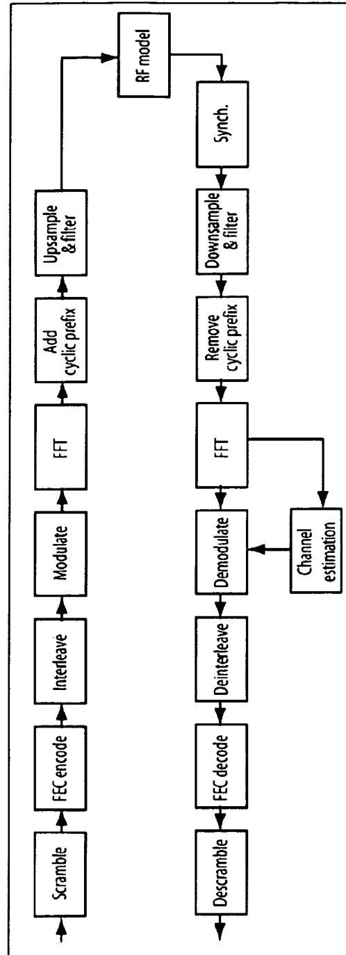
Figure 10 Conventional OFDM PHY system model
