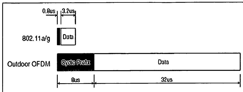
Figure 9 OFDM symbol dimensions
