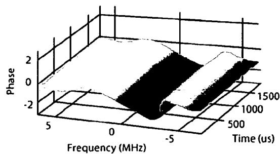
(a) Phase
