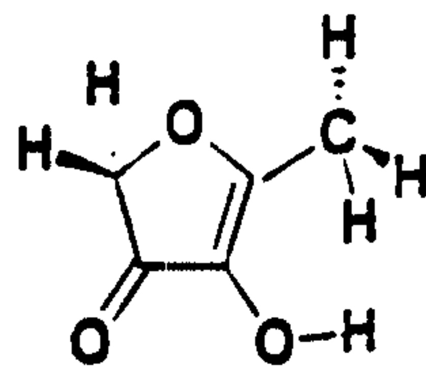
4-hydroxy-5-methyl-3(2H)-furanone
