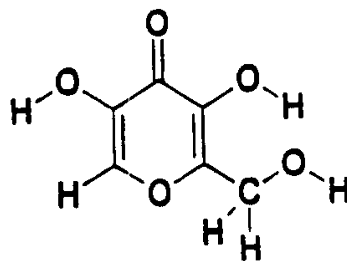
3-hydroxy-kojic acid
