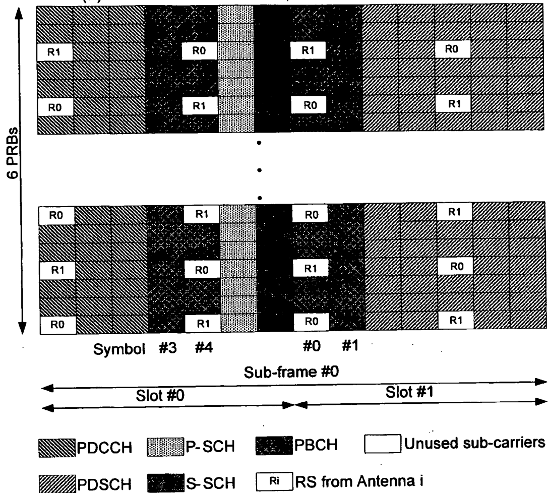
(B) – Current PBCH structure, 2 TX antennas at eNB, normal CP
