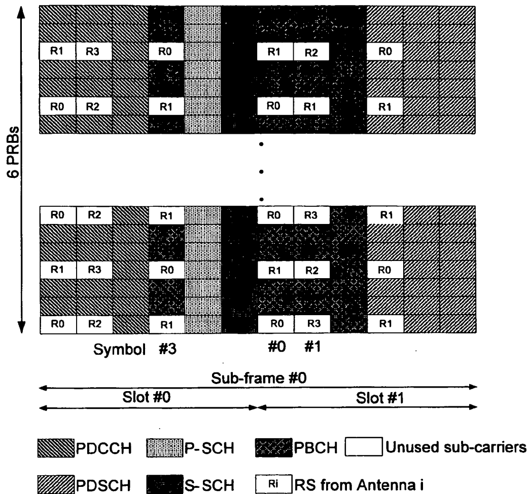
(C) – Current PBCH structure, 4 TX antenna at eNB, extended CP
