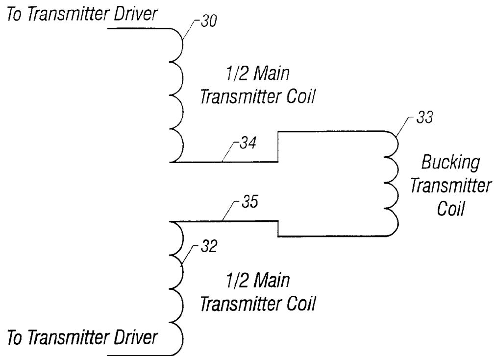
TILT Dual Transmitter Coil Arrangement
