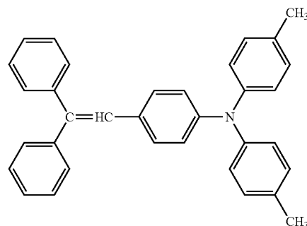
Chemical Structure (I)
