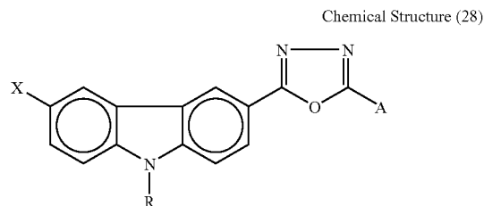
Chemical Structure (28)
