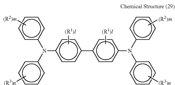
Chemical Structure (29)
