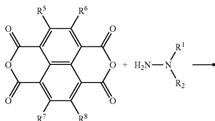
Chemical Reaction (III-1)
