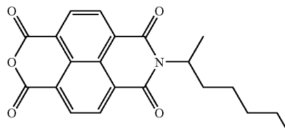
Chemical Structure (b)
