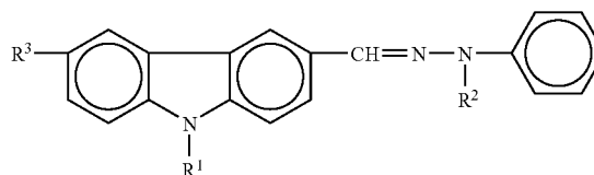
Chemical Structure (11)
