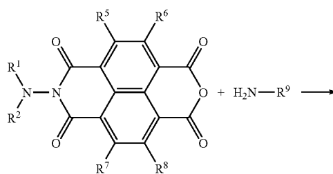
Chemical Reaction (III-2)
