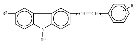
Chemical Structure (20)
