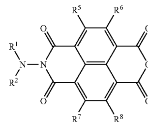
Chemical Reaction (III-2)
