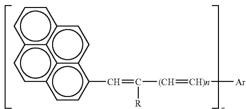
Chemical Structure (34)
