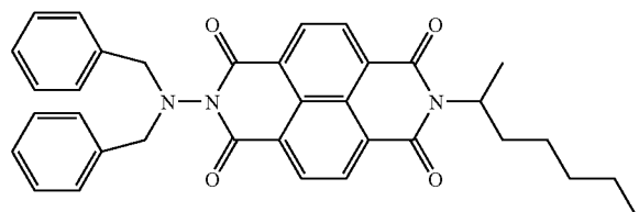
Chemical Structure (c)
