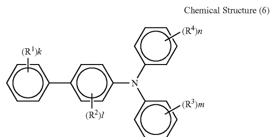
Chemical Structure (6)
