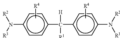
Chemical Structure (14)
