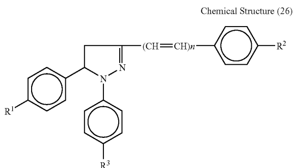
Chemical Structure (26)
