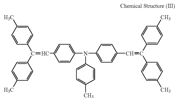
Chemical Structure (III)
