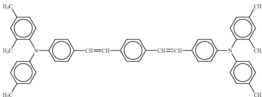
Examples 87 to 89
