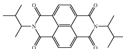
Chemical Structure (IX)
