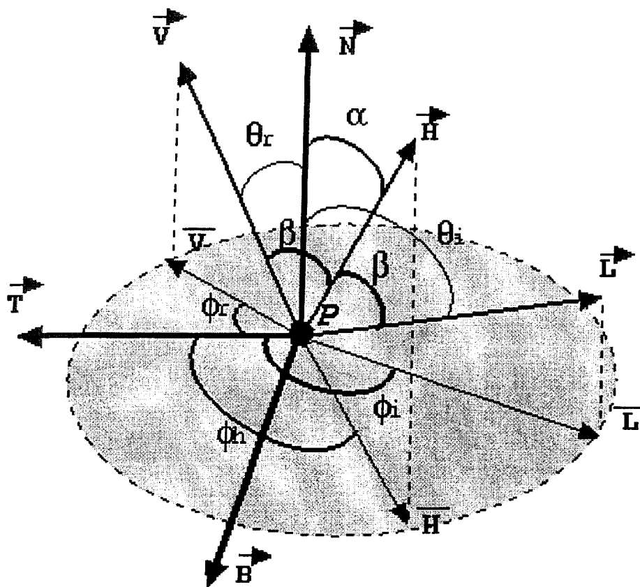
Figure 1: BRDF parameter definition
