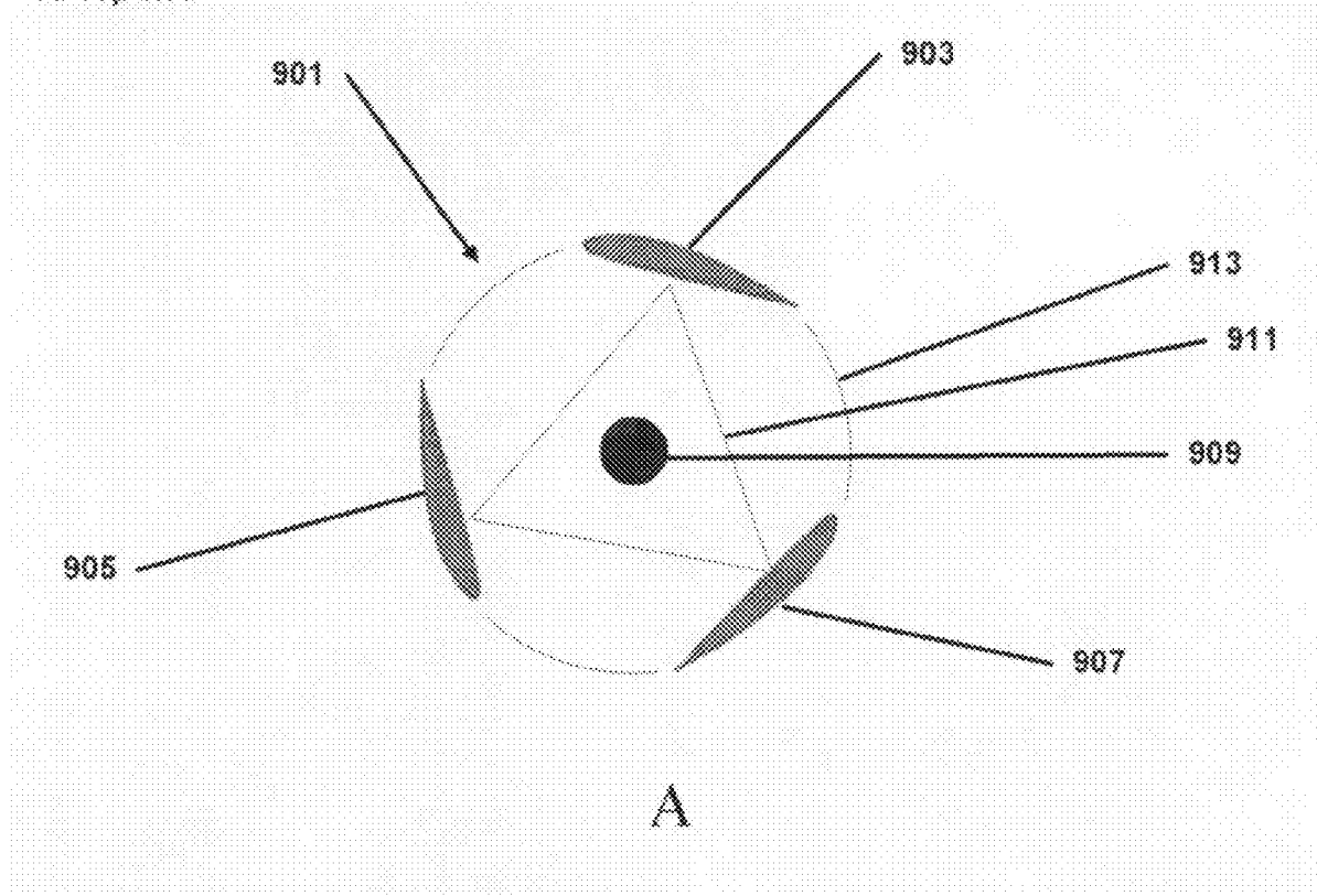
FIG. 5. Schematic Cross Sectional Diagram of a Vertical Wind Turbine Power Generating Module
