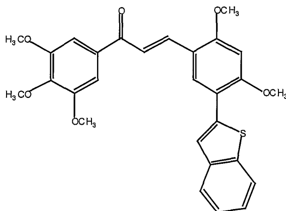
3-[5-(benzo[b]thien-2-yl)-2,4-dimethoxyphenyl]-1-(3,4,5-trimethoxyphenyl)- 2-propen-1-one
