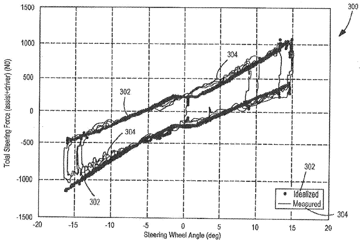
Idealized vs. Measured Rack Load
