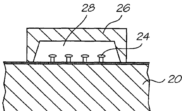
FIG. 3 (Prior Art)
