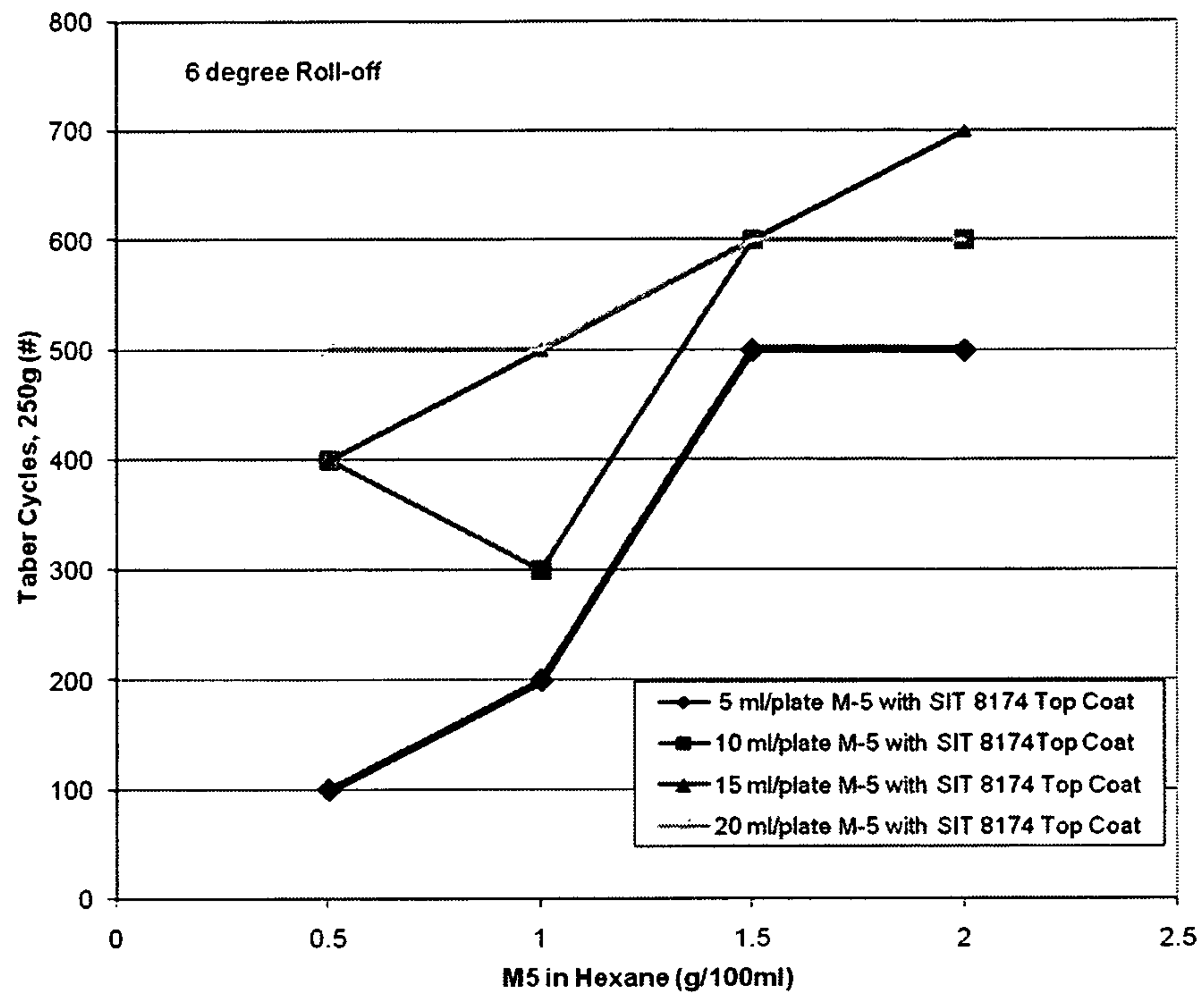
Figure 3: Taber cycles as affected by concentration of M5 and the amount of M5 used per 4- × 4-in. aluminum plate.
