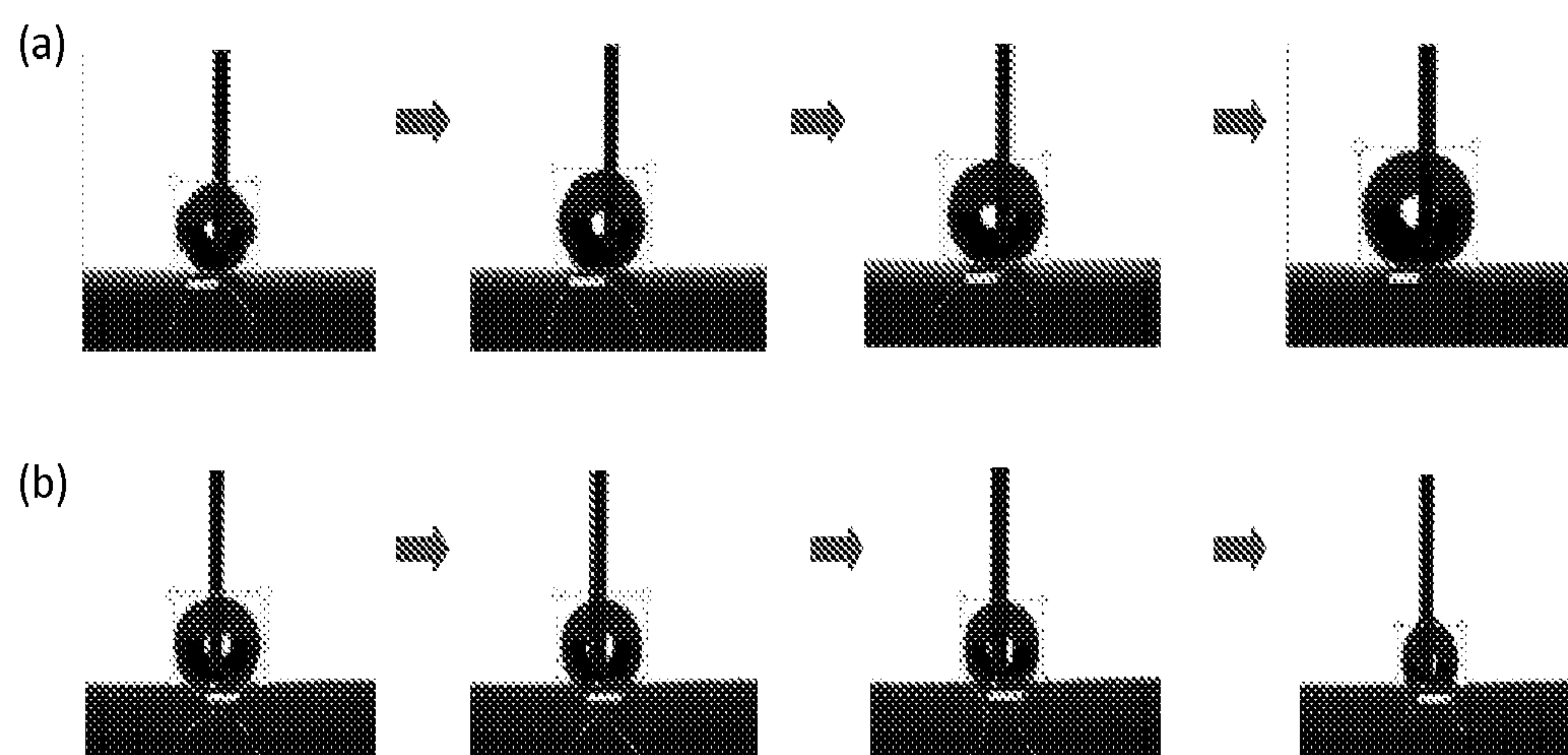
Figure 29: Captured images of advancing and receding water droplets on SH-coated samples (25-1000U): (a) advancing droplet and (b) receding droplet.
