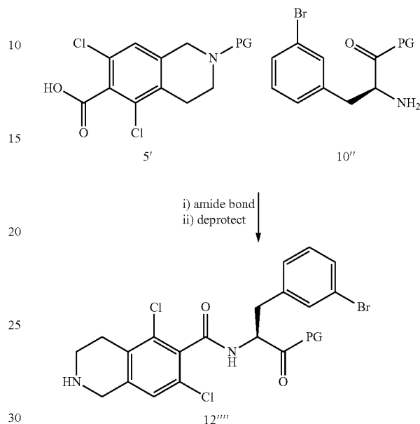
Scheme 3A
