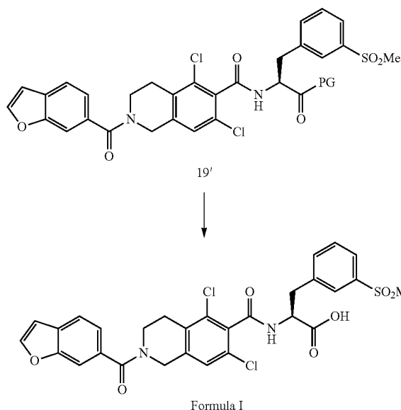
Formula I
