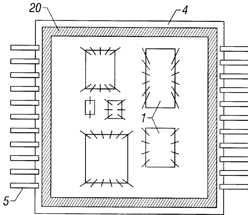
TOP VIEW
