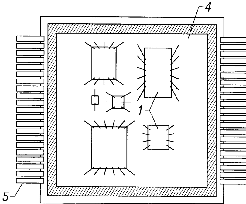
TOP VIEW
