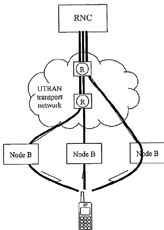
Macro diversity in the RNC
