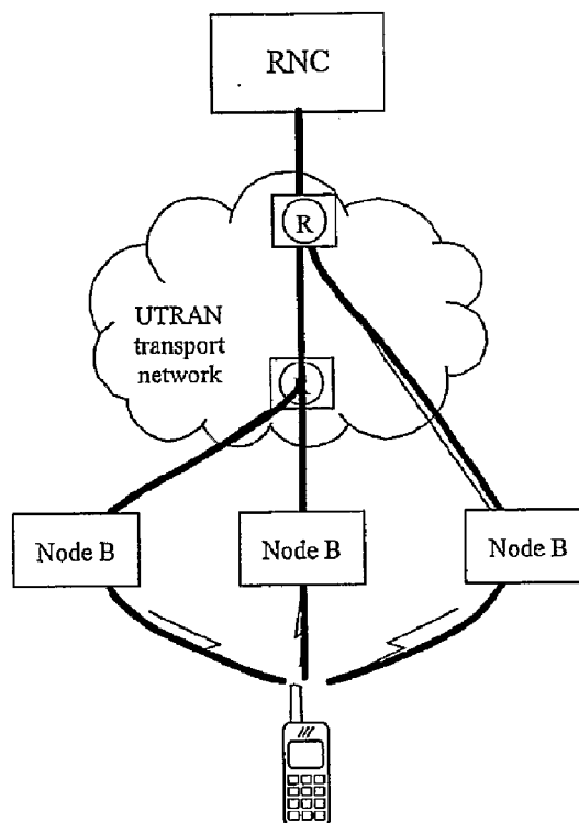
Macro diversity in the routers
