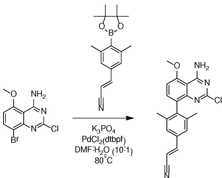
Compound 28c
