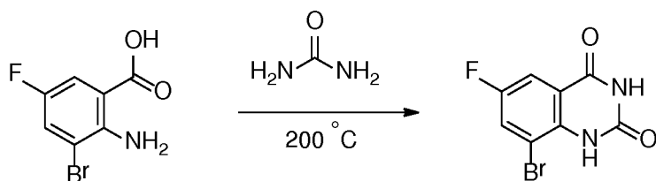
Compound 20b
