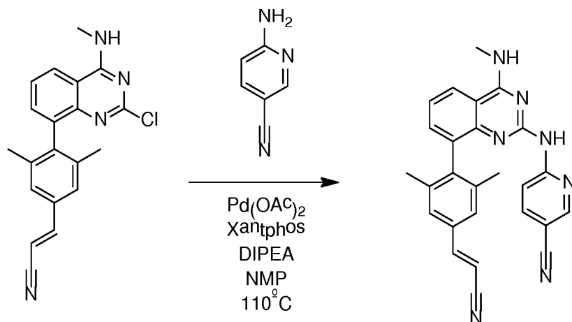
Compound 31
