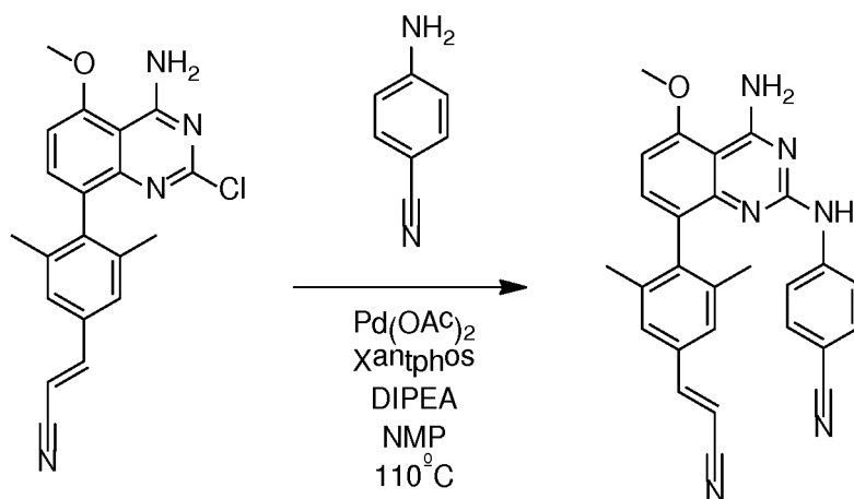
Compound 28
