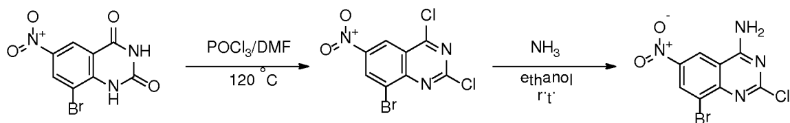
Compound 22c
