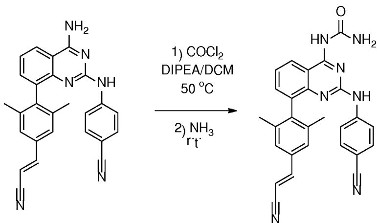
Compound 37
