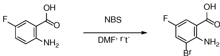
Compound 20a
