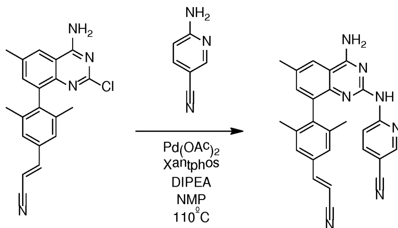
Compound 21
