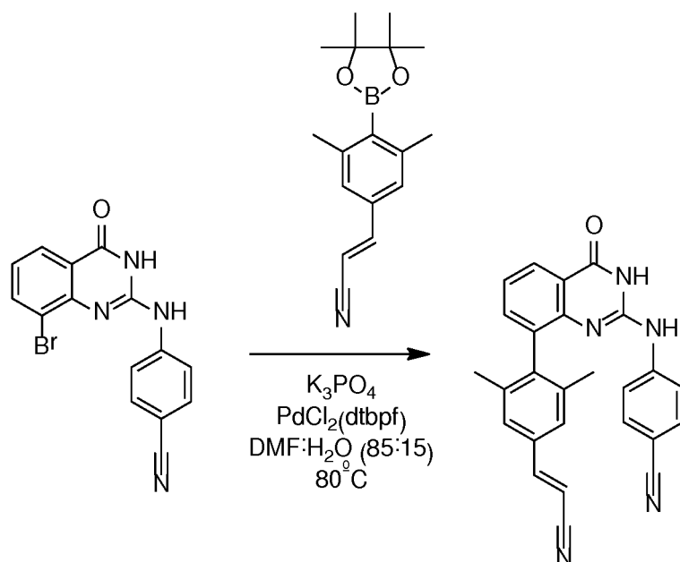
Compound 41
