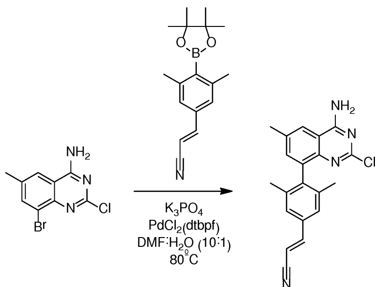
Compound 21d
