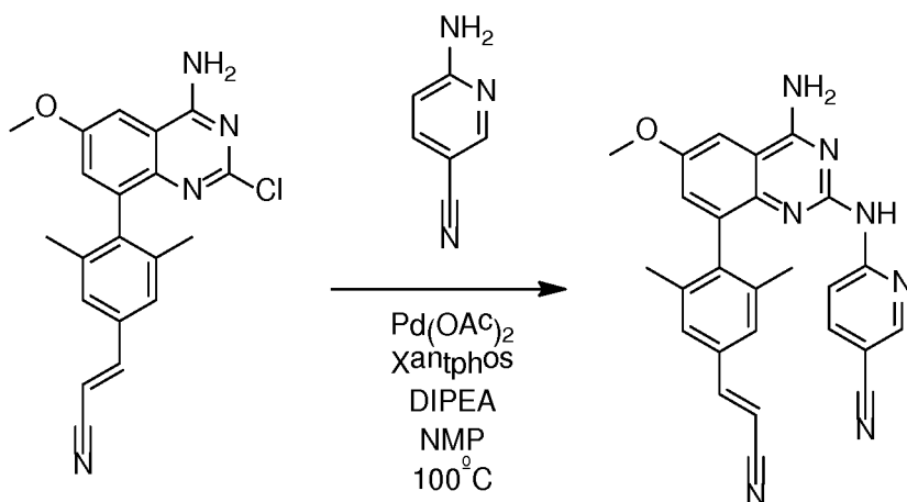
Compound 24
