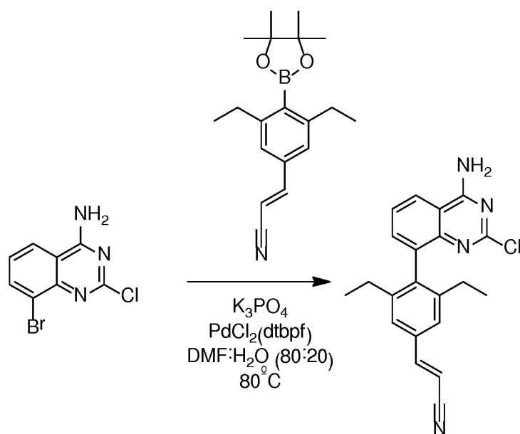
Compound 35c
