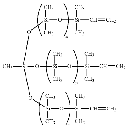
Vinyl Functional Q Branched (Left) and T Branched (Right) (Poly)Siloxane Precursors
