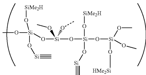
Hydride Functional Q Branched (Poly)Siloxane Precursor (HTS)
