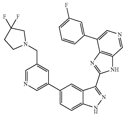
2-(5-(5-((3,3-Difluoropyrrolidin-1-yl)methyl)pyridin-3-yl)-1H-indazol-3-yl)-7-(3-fluorophenyl)-3H-imidazo[4,5-c]pyridine 336
