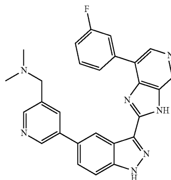
1-(5-(3-(7-(3-Fluorophenyl)-3H-imidazo[4,5-c]pyridin-2-yl)-1H-indazol-5-yl)pyridin-3-yl)-N,N-dimethylmethanamine 89
