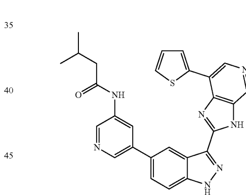
3-Methyl-N-(5-(3-(7-(thiophen-2-yl)-3H-imidazo[4,5-c]pyridin-2-yl)-1H-indazol-5-yl)pyridin-3-yl)butanamide 397
