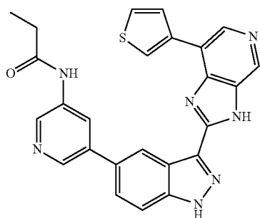
N-(5-(3-(7-(Thiophen-3-yl)-3H-imidazo[4,5-c]pyridin-2-yl)-1H-indazol-5-yl)pyridin-3-yl)propionamide 289
