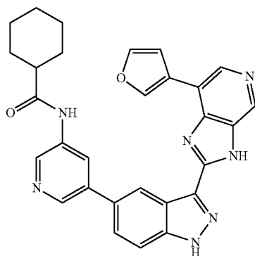
N-(5-(3-(7-(Furan-3-yl)-3H-imidazo[4,5-c]pyridin-2-yl)-1H-indazol-5-yl)pyridin-3-yl)cyclohexanecarboxamide 333
