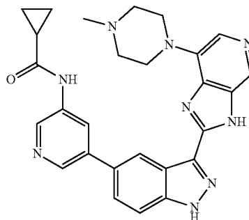
N-(5-(3-(7-(4-Methylpiperazin-1-yl)-3H-imidazo[4,5-c]pyridin-2-yl)-1H-indazol-5-yl)pyridin-3-yl)cyclopropanecarboxamide 260
