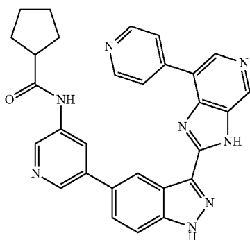
N-(5-(3-(7-(Pyridin-4-yl)-3H-imidazo[4,5-c]pyridin-2-yl)-1H-indazol-5-yl)pyridin-3-yl)cyclopentanecarboxamide 170
