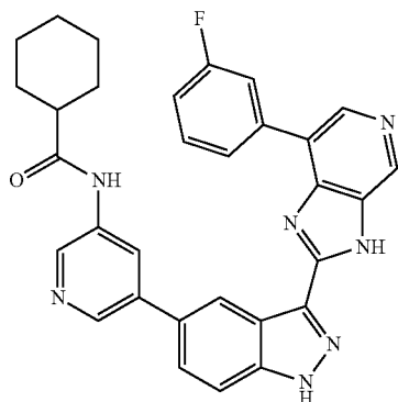
N-(5-(3-(7-(3-Fluorophenyl)-3H-imidazo[4,5-c]pyridin-2-yl)-1H-indazol-5-yl)pyridin-3-yl)cyclohexanecarboxamide 94
