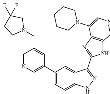
2-(5-(5-((3,3-Difluoropyrrolidin-1-yl)methyl)pyridin-3-yl)-1H-indazol-3-yl)-7-(piperidin-1-yl)-3H-imidazo[4,5-c]pyridine 342
