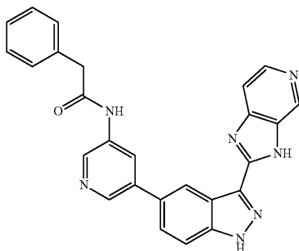
N-(5-(3-(3H-Imidazo[4,5-c]pyridin-2-yl)-1H-indazol-5-yl)pyridin-3-yl)-2-phenylacetamide 274
