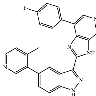
7-(4-Fluorophenyl)-2-(5-(4-methylpyridin-3-yl)-1H-indazol-3-yl)-3H-imidazo[4,5-c]pyridine 99
