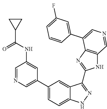
N-(5-(3-(7-(3-Fluorophenyl)-3H-imidazo[4,5-c]pyridin-2-yl)-1H-indazol-5-yl)pyridin-3-yl)cyclopropanecarboxamide 91
