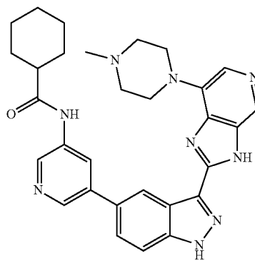
N-(5-(3-(7-(4-Methylpiperazin-1-yl)-3H-imidazo[4,5-c]pyridin-2-yl)-1H-indazol-5-yl)pyridin-3-yl)cyclohexanecarboxamide 263
