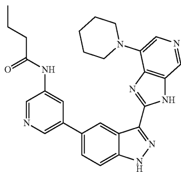
N-(5-(3-(7-(Piperidin-1-yl)-3H-imidazo[4,5-c]pyridin-2-yl)-1H-indazol-5-yl)pyridin-3-yl)butyramide 214
