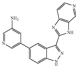
5-(3-(3H-Imidazo[4,5-c]pyridin-2-yl)-1H-indazol-5-yl)pyridin-3-amine 268
