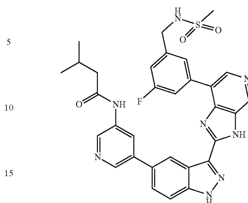
N-(5-(3-(7-(3-Fluoro-5-(methylsulfonamidomethyl)phenyl)-3H-imidazo[4,5-c]pyridin-2-yl)-1H-indazol-5-yl)pyridin-3-yl)-3-methylbutanamide 373
