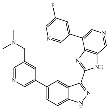
1-(5-(3-(7-(5-fluoropyridin-3-yl)-3H-imidazo[4,5-c]pyridin-2-yl)-1H-indazol-5-yl)pyridin-3-yl)-N,N-dimethylmethanamine 16
