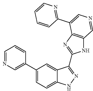
7-(Pyridin-2-yl)-2-(5-(pyridin-3-yl)-1H-indazol-3-yl)-3H-imidazo[4,5-c]pyridine 177
