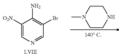
Scheme 13
