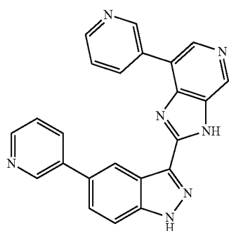
7-(Pyridin-3-yl)-2-(5-(pyridin-3-yl)-1H-indazol-3-yl)-3H-imidazo[4,5-c]pyridine 136
