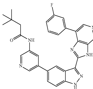
N-(5-(3-(7-(3-Fluorophenyl)-3H-imidazo[4,5-c]pyridin-2-yl)-1H-indazol-5-yl)pyridin-3-yl)-3,3-dimethylbutanamide 90
