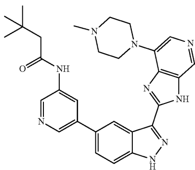
3,3-Dimethyl-N-(5-(3-(7-(4-methylpiperazin-1-yl)-3H-imidazo[4,5-c]pyridin-2-yl)-1H-indazol-5-yl)pyridin-3-yl)butanamide 257
