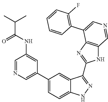
N-(5-(3-(7-(2-Fluorophenyl)-3H-imidazo[4,5-c]pyridin-2-yl)-1H-indazol-5-yl)pyridin-3-yl)isobutyramide 31
