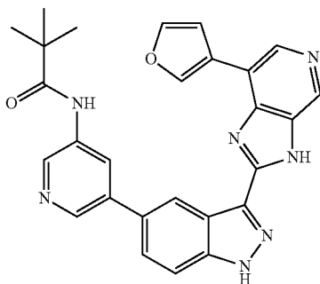
N-(5-(3-(7-(Furan-3-yl)-3H-imidazo[4,5-c]pyridin- 2-yl)-1H-indazol-5-yl)pyridin-3-yl)pivalamide 319
