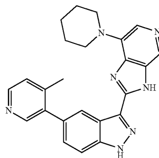
2-(5-(4-Methylpyridin-3-yl)-1H-indazol-3-yl)-7-(piperidin-1-yl)-3H-imidazo[4,5-c]pyridine 202
