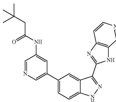
N-(5-(3-(3H-Imidazo[4,5-c]pyridin-2-yl)-1H-indazol-5-yl)pyridin-3-yl)-3,3-dimethylbutanamide 280
