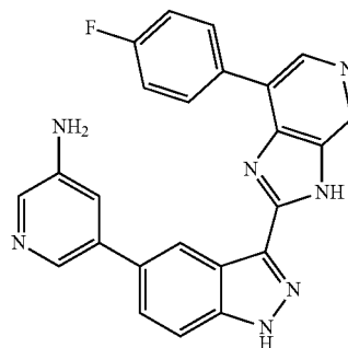
5-(3-(7-(4-Fluorophenyl)-3H-imidazo[4,5-c]pyridin-2-yl)-1H-indazol-5-yl)pyridin-3-amine 97
