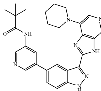
N-(5-(3-(7-(Piperidin-1-yl)-3H-imidazo[4,5-c]pyridin-2-yl)-1H-indazol-5-yl)pyridin-3-yl)pivalamide 205
