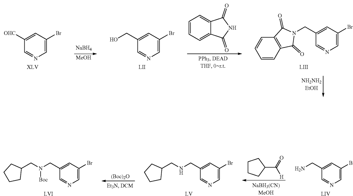
Scheme 11
