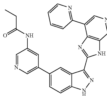
N-(5-(3-(7-(Pyridin-2-yl)-3H-imidazo[4,5-c]pyridin-2-yl)-1H-indazol-5-yl)pyridin-3-yl)propionamide 174
