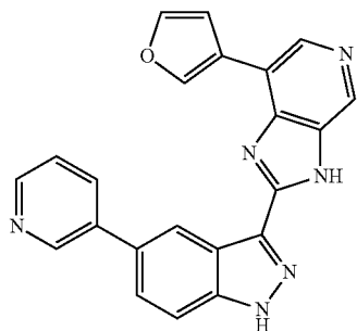
7-(Furan-3-yl)-2-(5-(pyridin-3-yl)-1H-indazol-3-yl)- 3H-imidazo[4,5-c]pyridine 315
