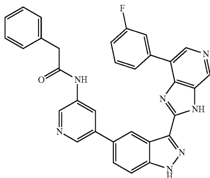
N-(5-(3-(7-(3-Fluorophenyl)-3H-imidazo[4,5-c]pyridin-2-yl)-1H-indazol-5-yl)pyridin-3-yl)-2-phenylacetamide 86
