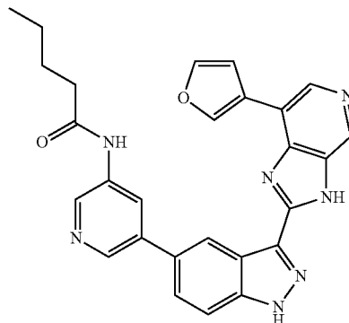
N-(5-(3-(7-(Furan-3-yl)-3H-imidazo[4,5-c]pyridin- 2-yl)-1H-indazol-5-yl)pyridin-3-yl)pentanamide 329
