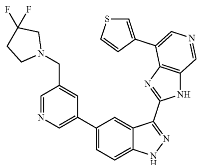
2-(5-((3,3-Difluoropyrrolidin-1-yl)methyl)pyridin-3-yl)-1H-indazol-3-yl)-7-(thiophen-3-yl)-3H-imidazo[4,5-c]pyridine 346
