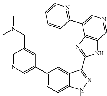
N,N-Dimethyl-1-(5-(3-(7-(pyridin-2-yl)-3H-imidazo[4,5-c]pyridin-2-yl)-1H-indazol-5-yl)pyridin-3-yl)methanamine 186
