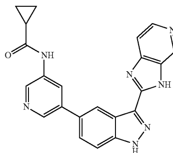
N-(5-(3-(3H-Imidazo[4,5-c]pyridin-2-yl)-1H-indazol-5-yl)pyridin-3-yl)cyclopropanecarboxamide 283
