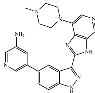
5-(3-(7-(4-Methylpiperazin-1-yl)-3H-imidazo[4,5-c]pyridin-2-yl)-1H-indazol-5-yl)pyridin-3-amine 247
