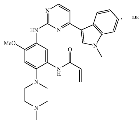
AZD9291
