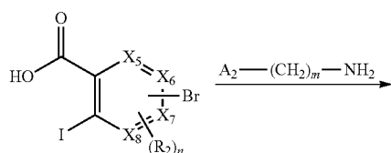
General Scheme 2
