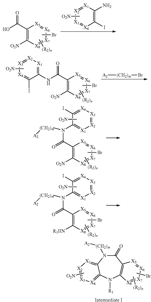
General Scheme 1
