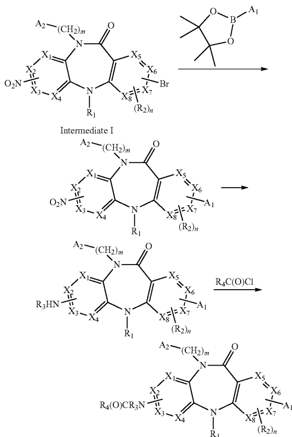
General Scheme 3
