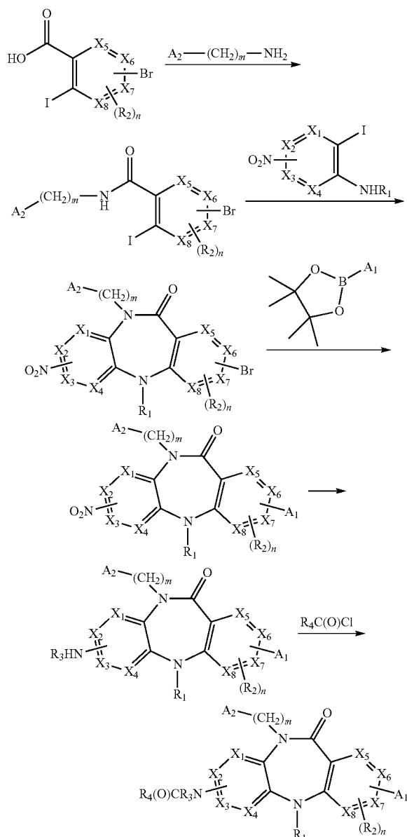
General Scheme 4
