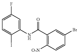
Step 1: 5-Bromo-N-(5-fluoro-2-iodophenyl)-2-nitrobenzamide [0571]
