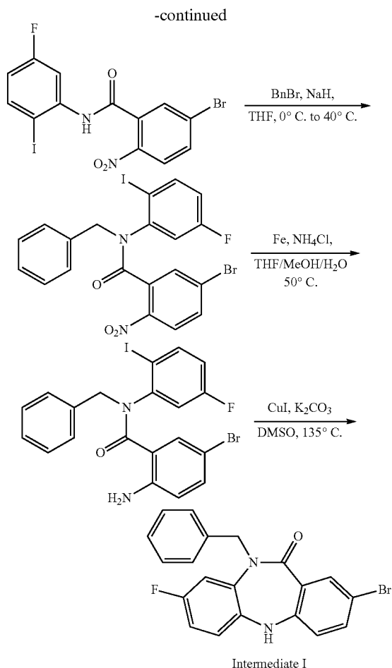
Step 1: 5-Bromo-N-(5-fluoro-2-iodophenyl)-2-nitrobenzamide [0571]
