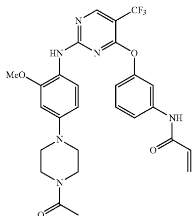
CO-1686
