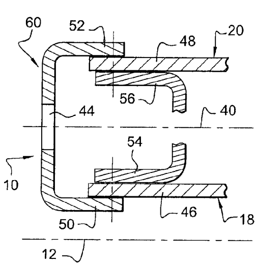
Fig. 2 Prior Art
