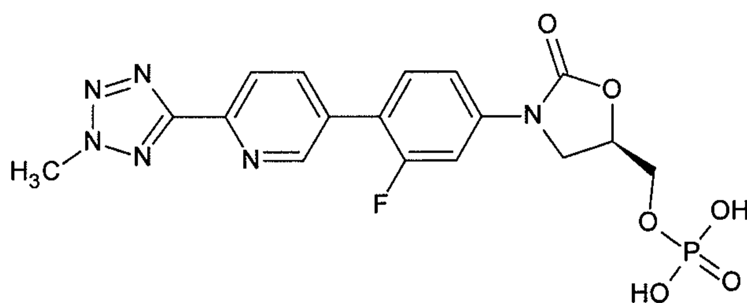
Formula IIa (M = OH).
