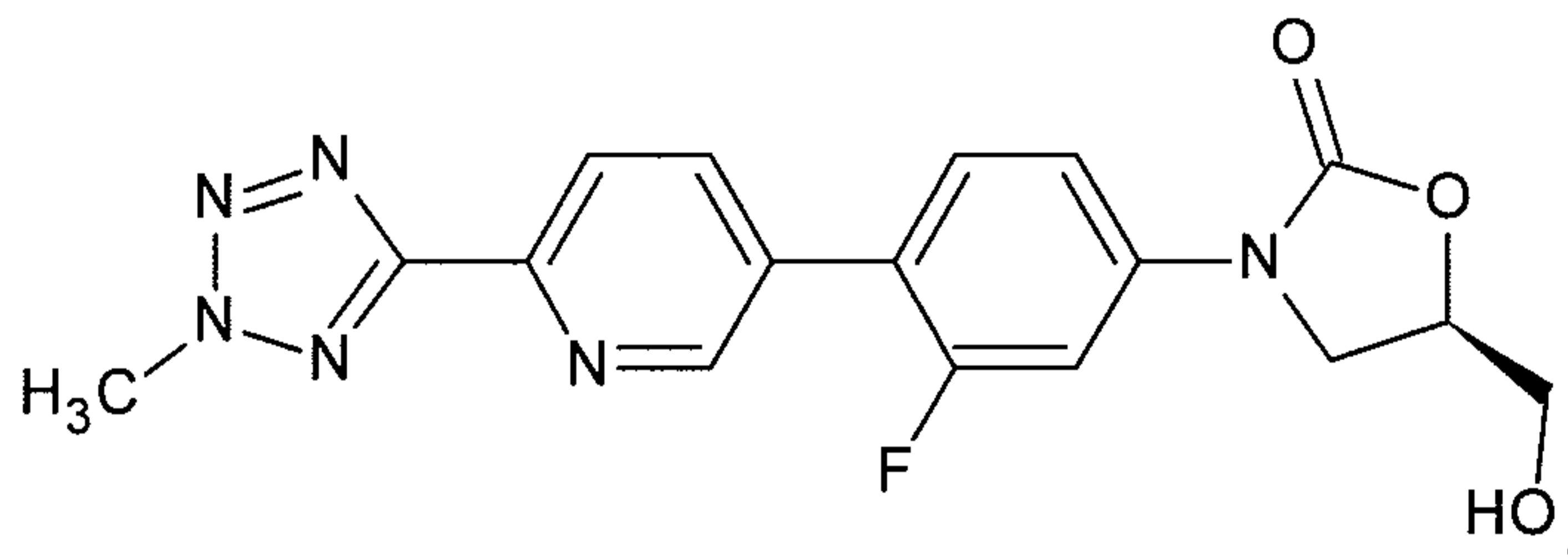
Formula Ia ("TR-700".)
