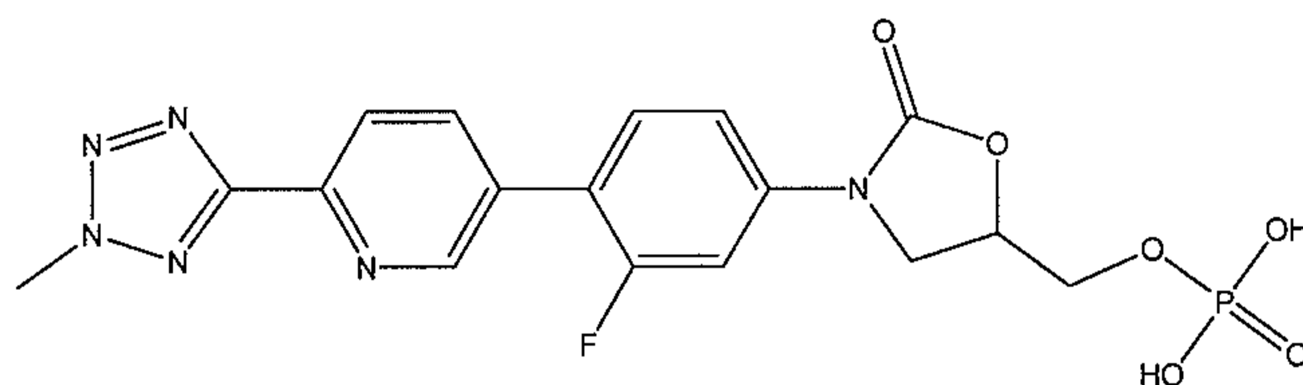
Formula II (M = OH).
