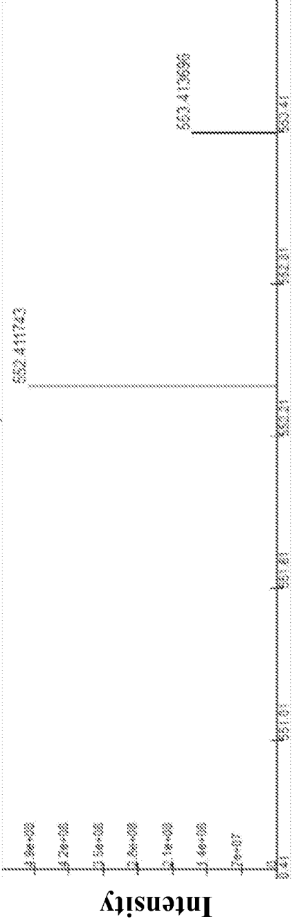
luminimide B
