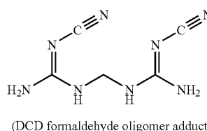
(DCD formaldehyde oligomer adduct)
