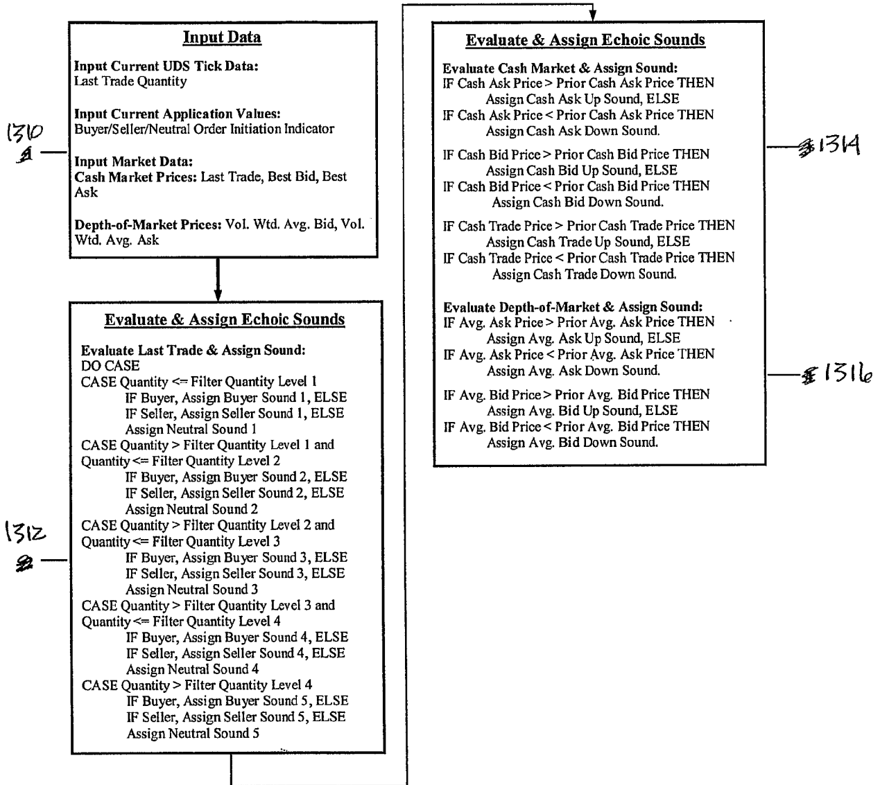
FIG. 13 – Process for Assigning Echoic Sounds to Transactions
