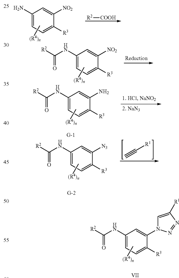
Reaction scheme G1
