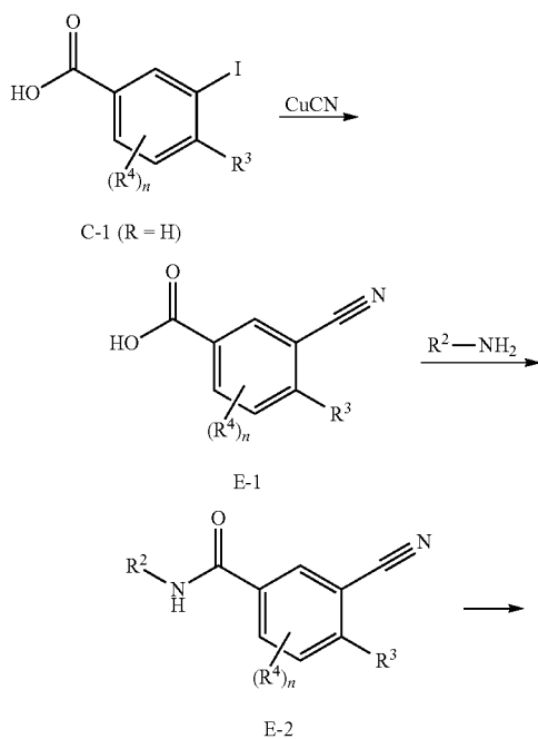
Reaction scheme E
