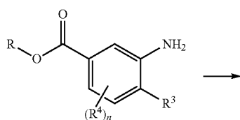
Reaction scheme C
