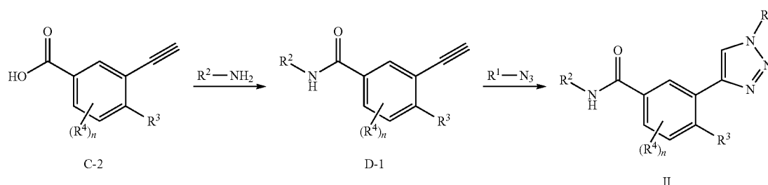
Reaction scheme D
