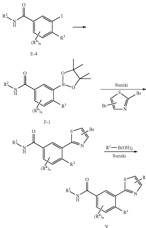
Reaction scheme F
