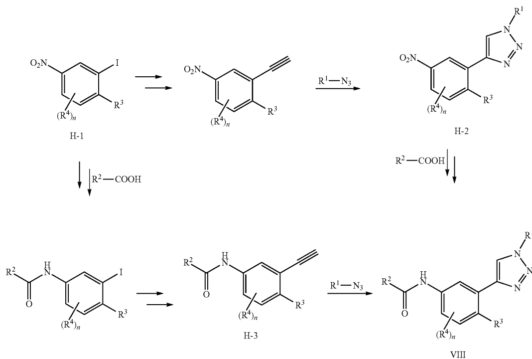
Reaction scheme H
