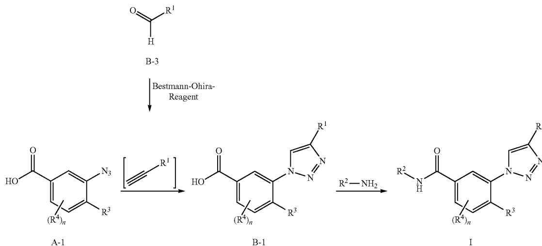
Reaction scheme B
