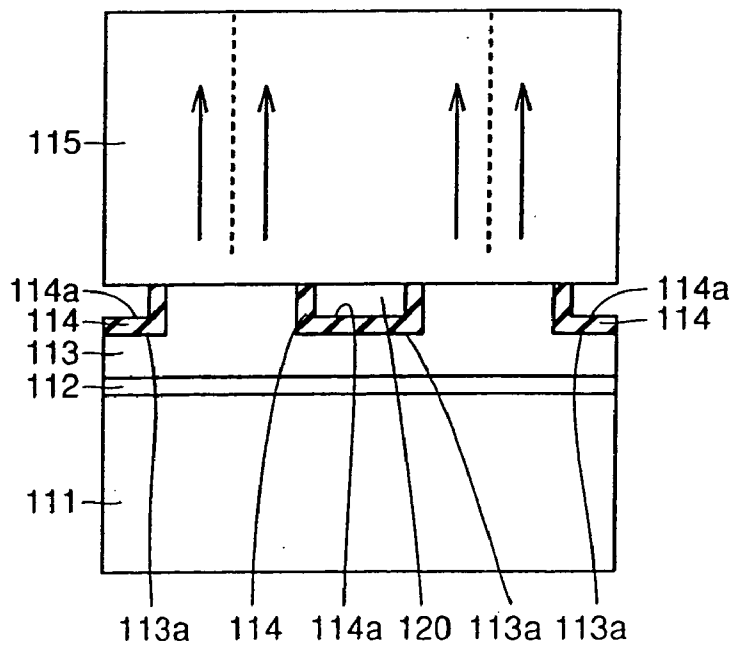
FIG.30 PRIOR ART
