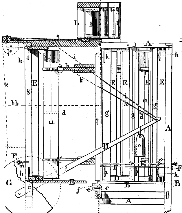
Fig. 1. Left div n is vert. sec. on line "aa" fig. 2. Right " " is an elevation.
