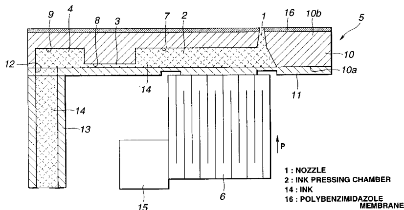
CROSS SECTIONAL VIEW OF PRINTING DEVICE
