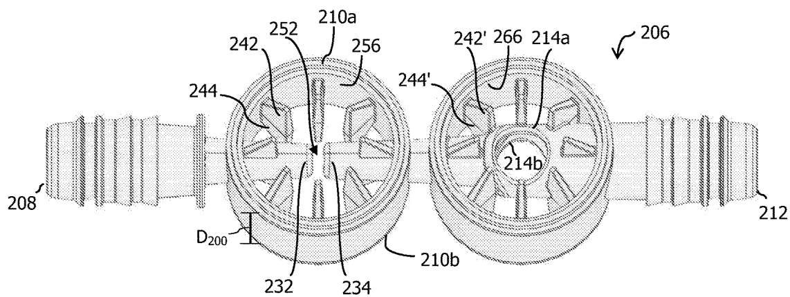
FIG. 3 (Prior Art)
