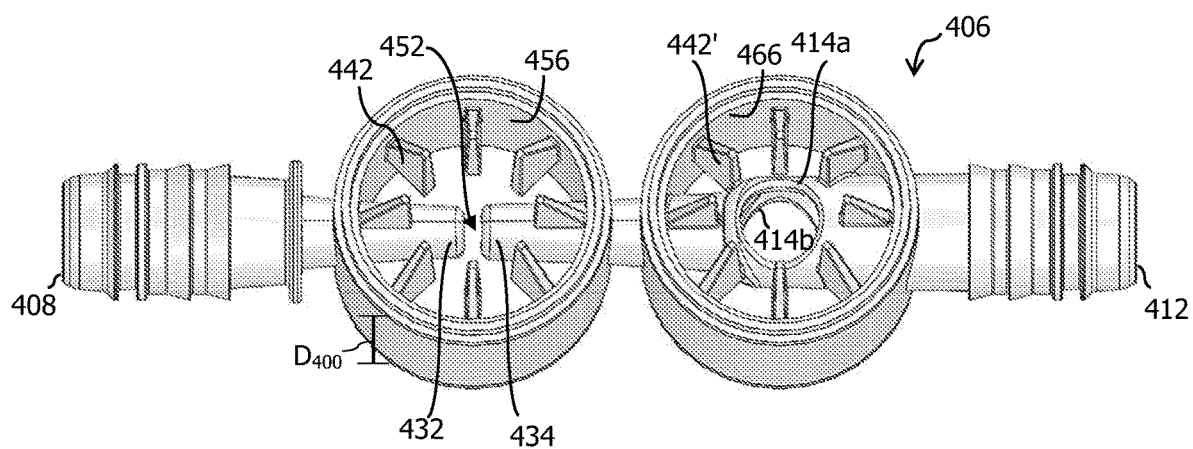
FIG. 5 (Prior Art)
